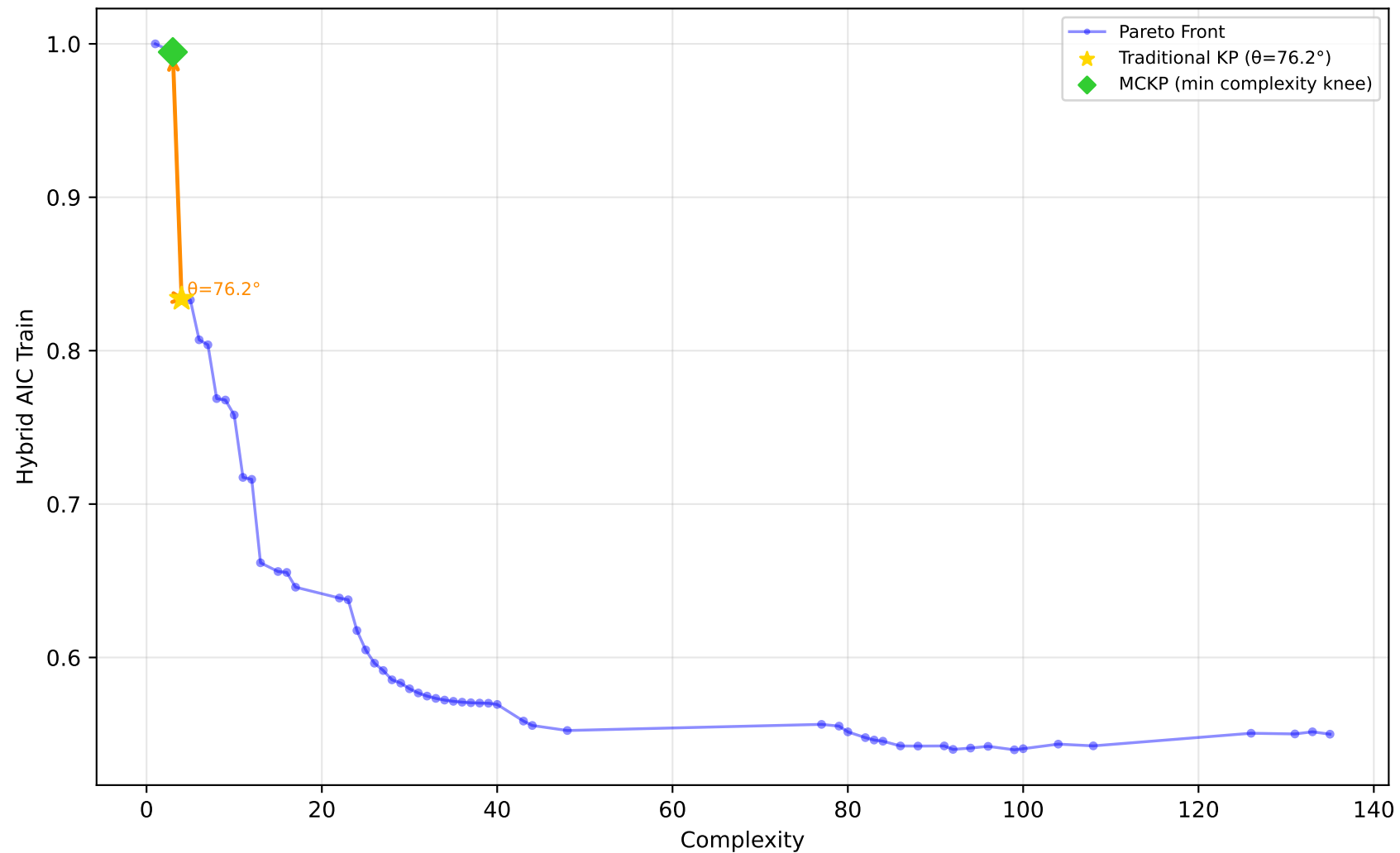
637_fri_c1_500_50 - Run 18 - SVP - Hybrid AIC Train \lambda_1=0.00, \lambda_2=0.00, \lambda_3=0.00 | Difficulty: 1.00 | Method: hmr
