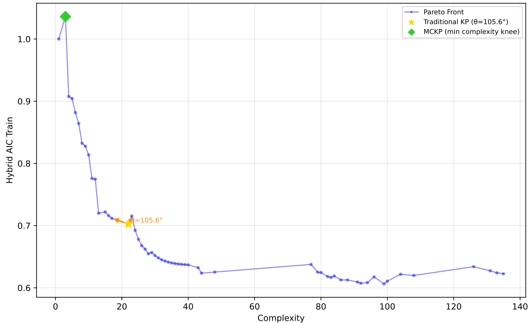
637_fri_c1_500_50 - Run 18 - SVP - Hybrid AIC Train \lambda_1=0.10, \lambda_2=0.00, \lambda_3=0.20 | Difficulty: 1.00 | Method: hmr
