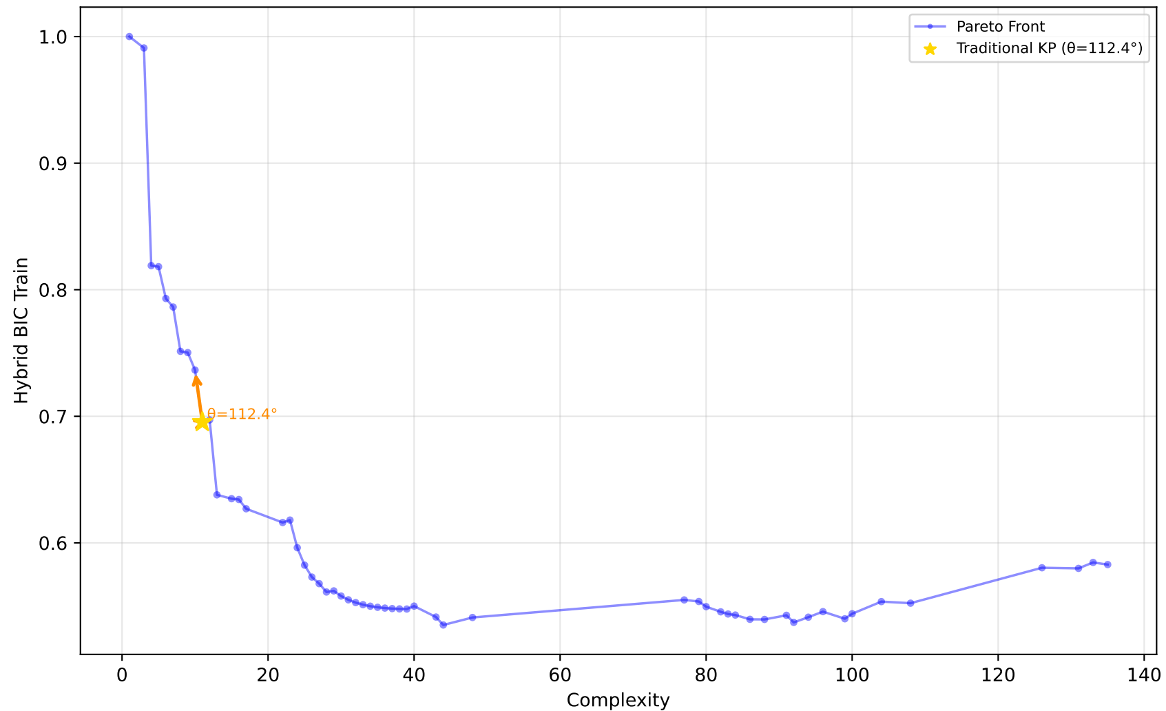
637_fri_c1_500_50 - Run 18 - SVP - Hybrid BIC Train \lambda_1=0.00, \lambda_2=0.00, \lambda_3=0.00 | Difficulty: 1.00 | Method: hmr
