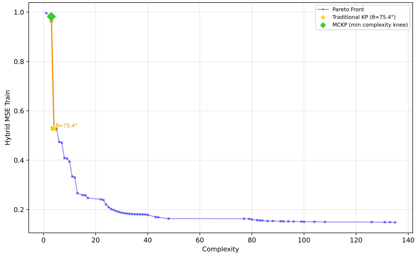
637_fri_c1_500_50 - Run 18 - SVP - Hybrid MSE Train \lambda_1=0.00, \lambda_2=0.00, \lambda_3=0.00 | Difficulty: 1.00 | Method: hmr
