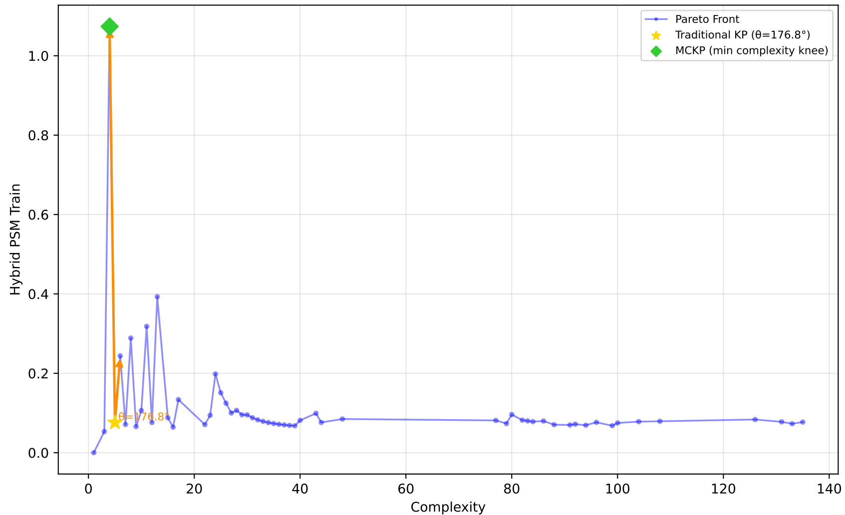
637_fri_c1_500_50 - Run 18 - SVP - Hybrid PSM Train \lambda_1=0.10, \lambda_2=0.00, \lambda_3=0.20 | Difficulty: 1.00 | Method: hmr
