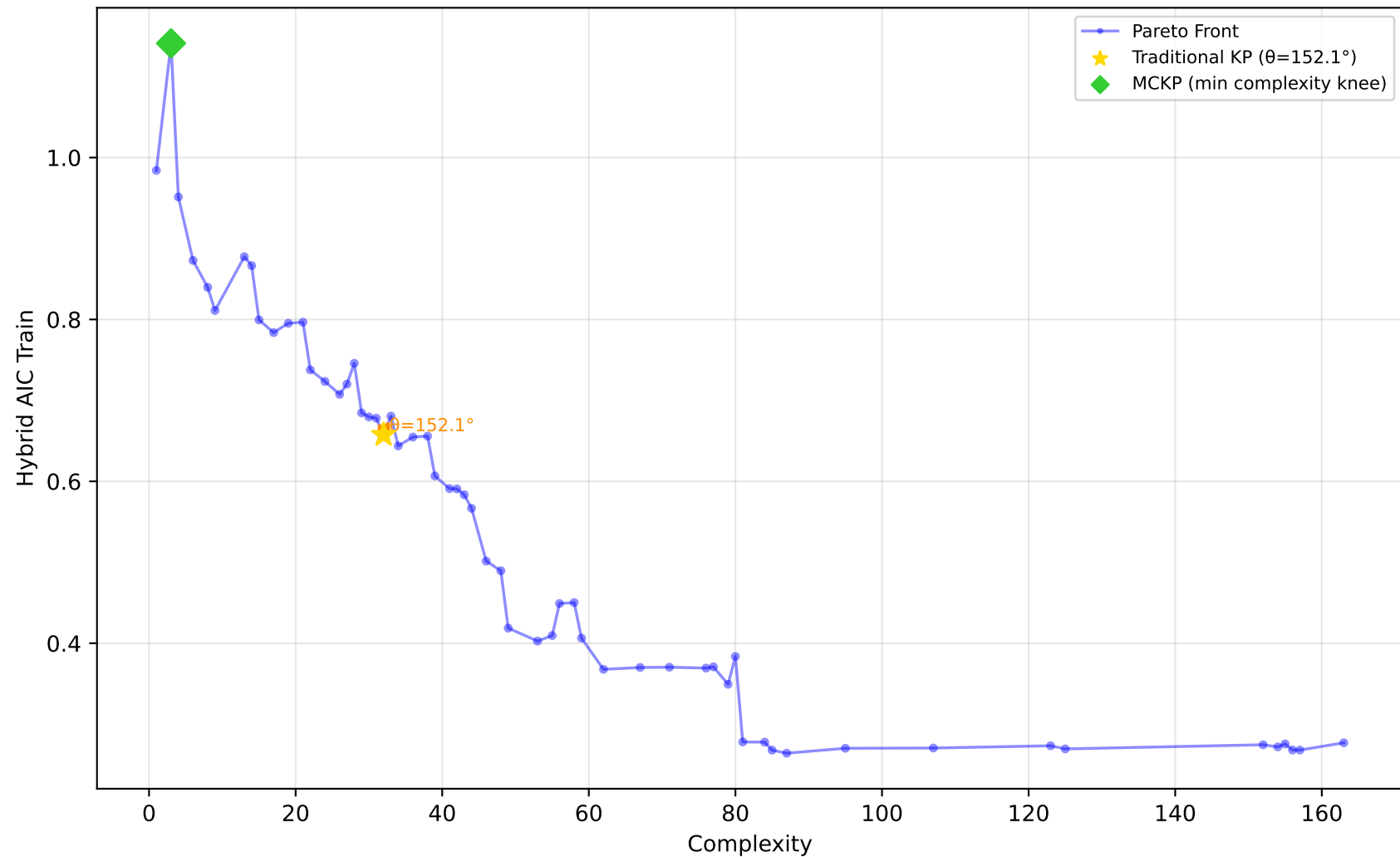
637_fri_c1_500_50 - Run 19 - MVP - Hybrid AIC Train \lambda_1=0.10, \lambda_2=0.00, \lambda_3=1.00 | Difficulty: 1.00 | Method: hmr
