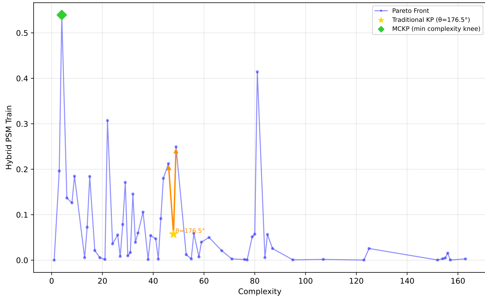
637_fri_c1_500_50 - Run 19 - MVP - Hybrid PSM Train \lambda_1=0.00, \bar{\lambda}_2=0.50, \lambda_3=0.00 | Difficulty: 1.00 | Method: hmr
