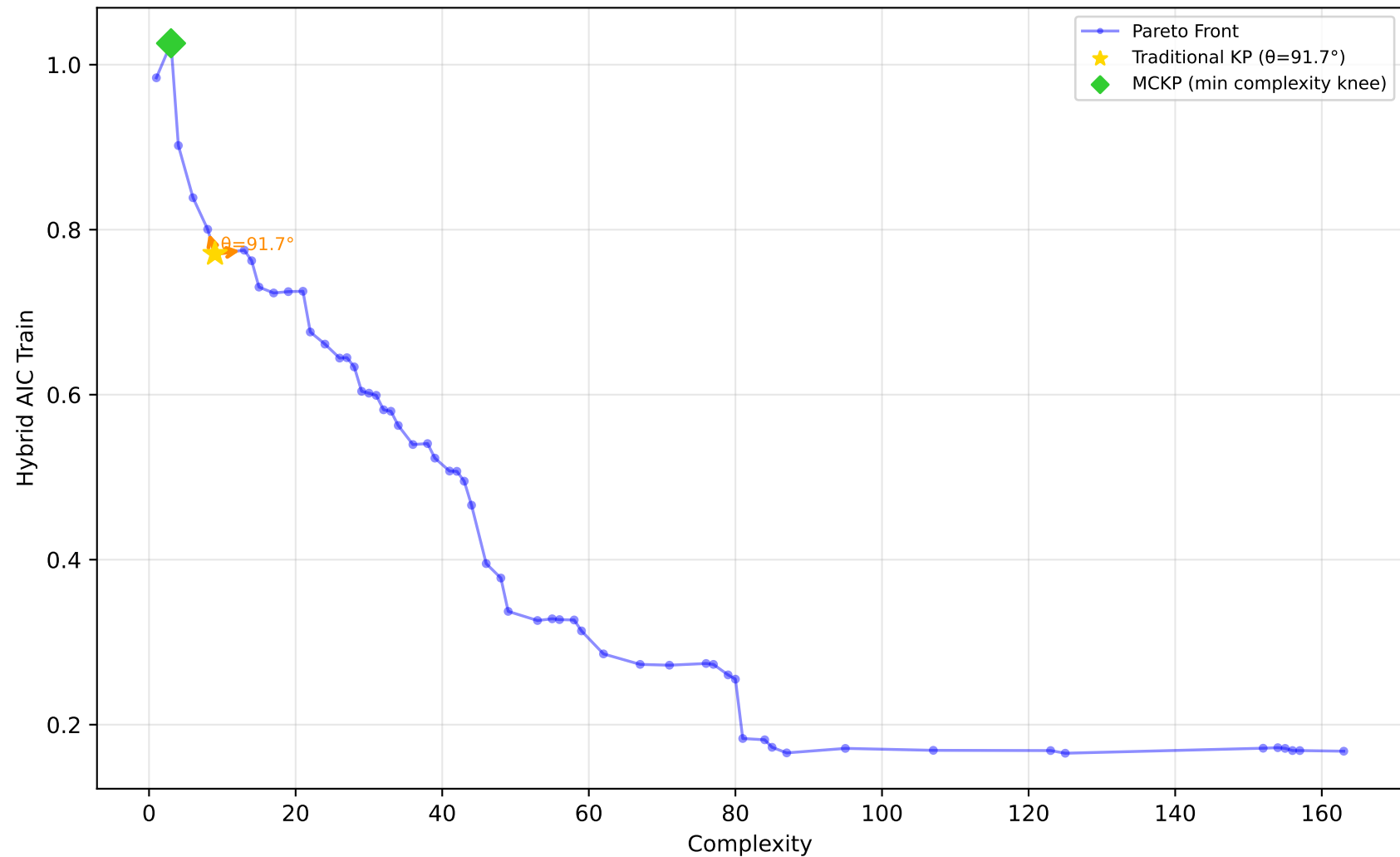
637_fri_c1_500_50 - Run 19 - SVP - Hybrid AIC Train \lambda_1=0.10, \lambda_2=0.00, \lambda_3=0.20 | Difficulty: 1.00 | Method: hmr
