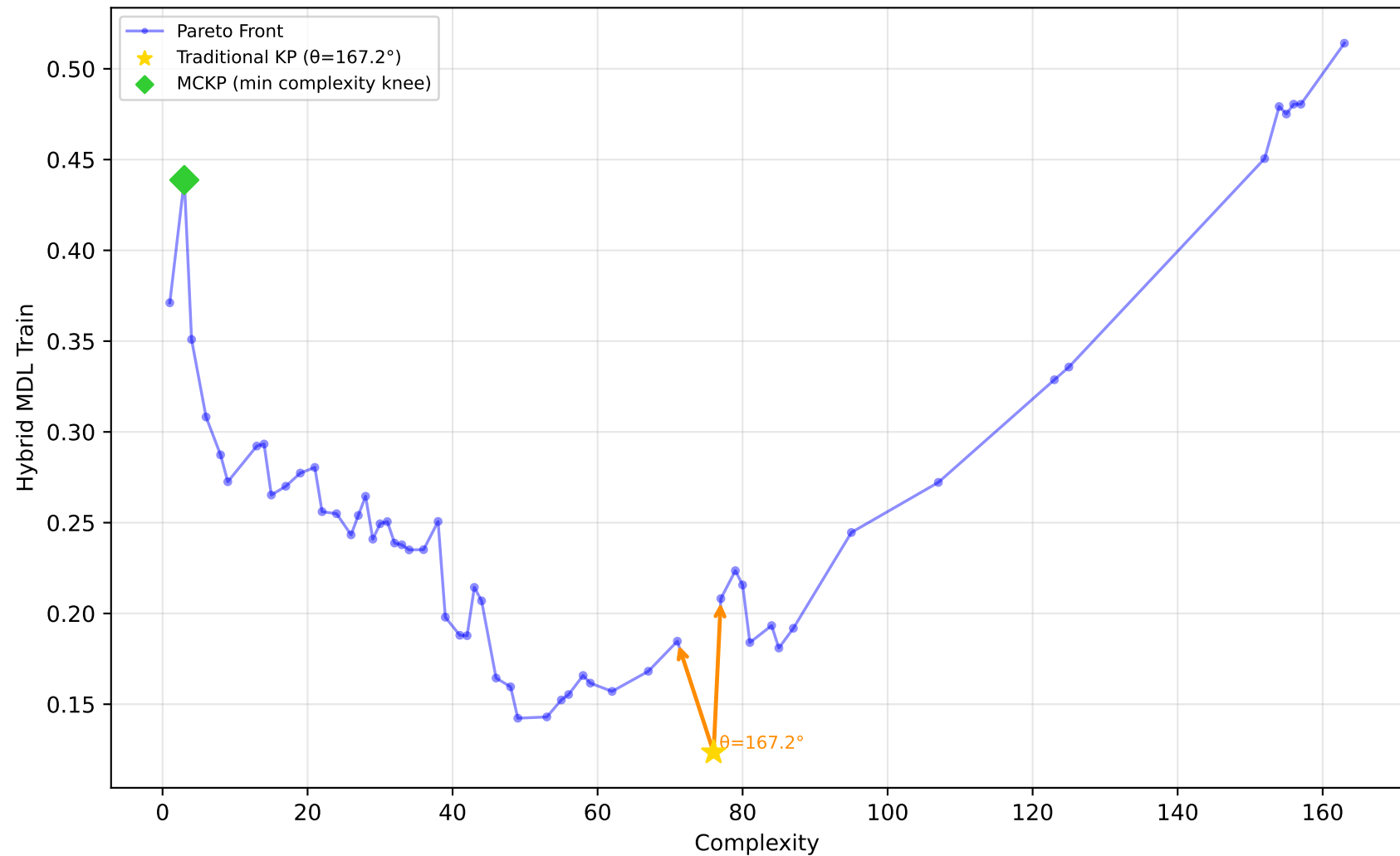
637_fri_c1_500_50 - Run 19 - SVP - Hybrid MDL Train \lambda_1=0.10, \lambda_2=0.00, \lambda_3=0.20 | Difficulty: 1.00 | Method: hmr
