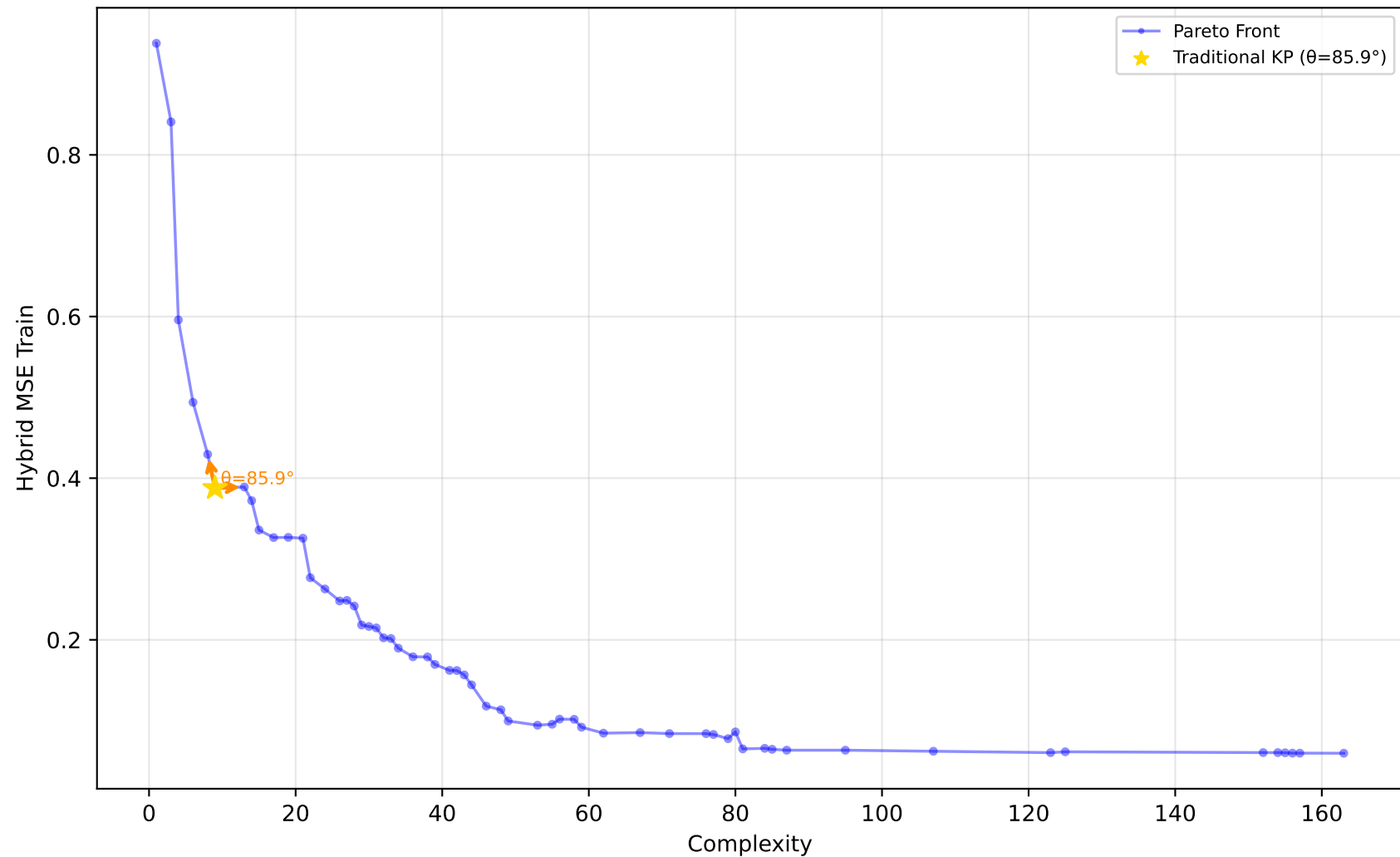
637_fri_c1_500_50 - Run 19 - SVP - Hybrid MSE Train \lambda_1=0.10, \lambda_2=0.00, \lambda_3=0.20 | Difficulty: 1.00 | Method: hmr
