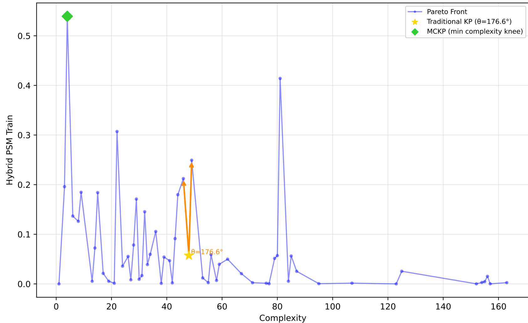
637_fri_c1_500_50 - Run 19 - SVP - Hybrid PSM Train \lambda_1=0.00, \lambda_2=0.00, \lambda_3=0.00 | Difficulty: 1.00 | Method: hmr
