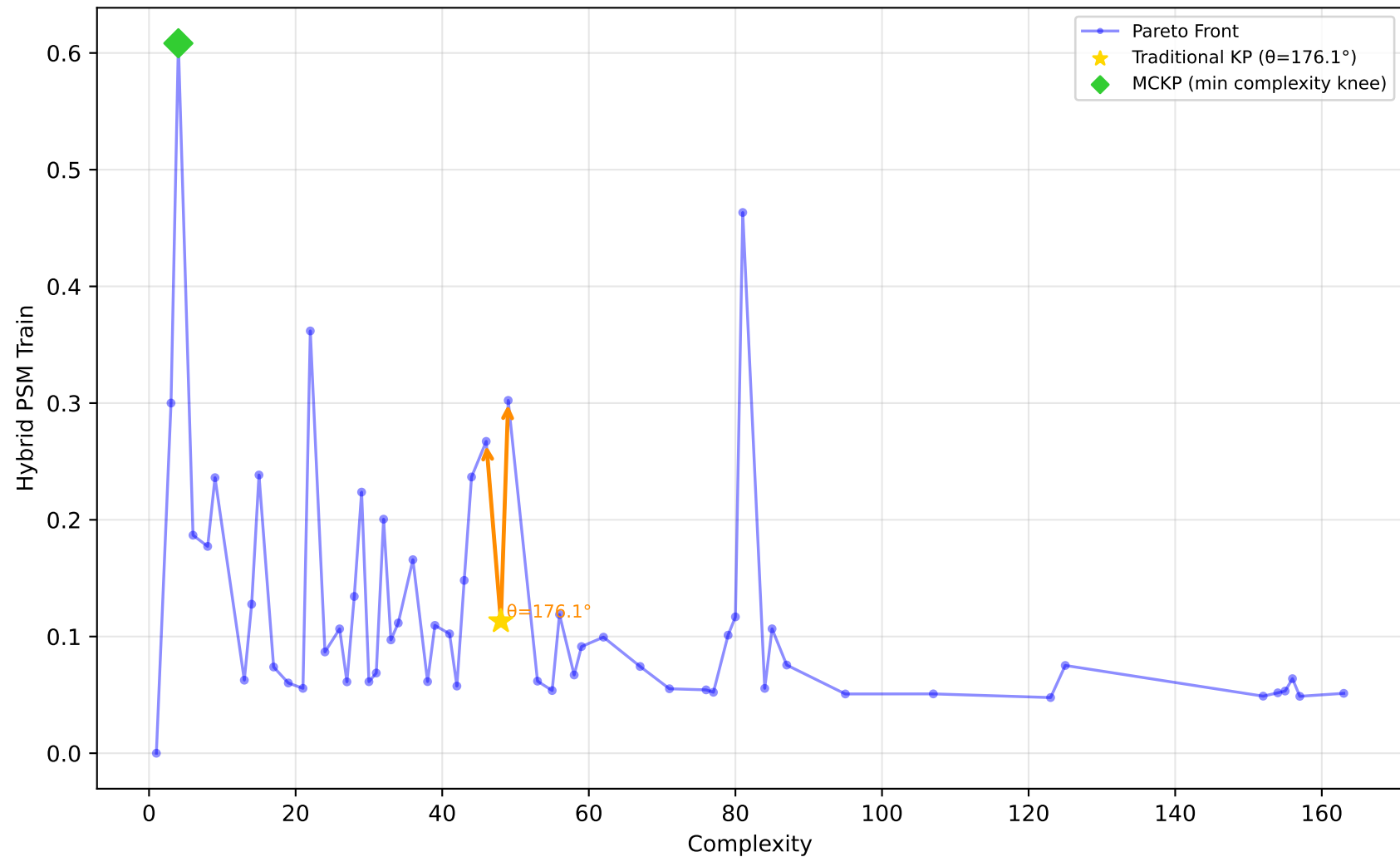
637_fri_c1_500_50 - Run 19 - SVP - Hybrid PSM Train \lambda_1=0.10, \lambda_2=0.00, \lambda_3=0.20 | Difficulty: 1.00 | Method: hmr
