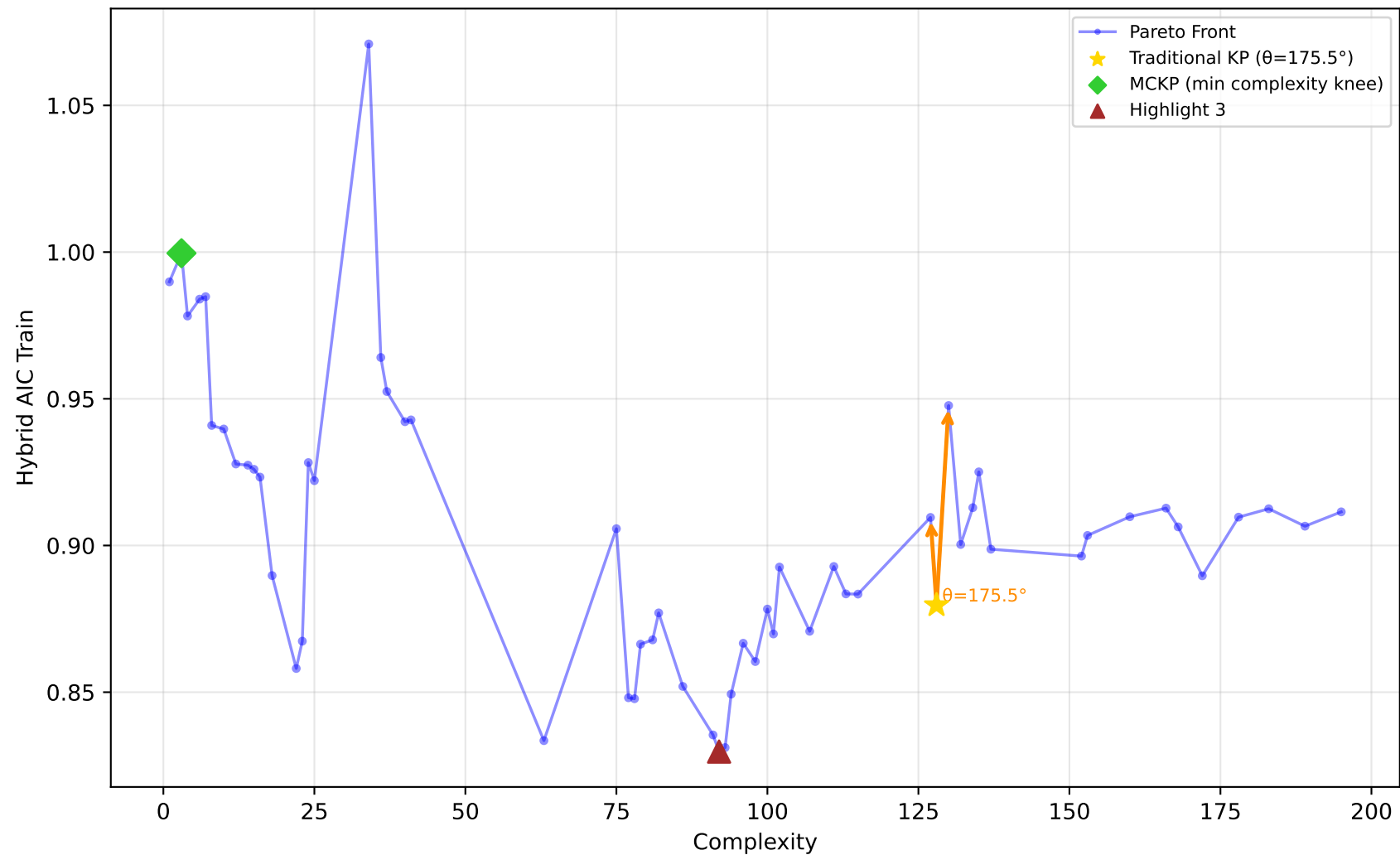
637_fri_c1_500_50 - Run 1 - MVP - Hybrid AIC Train \lambda_1=0.10 , \lambda_2=0.00 , \lambda_3=1.00 | Difficulty: 1.00 | Method: hmr
