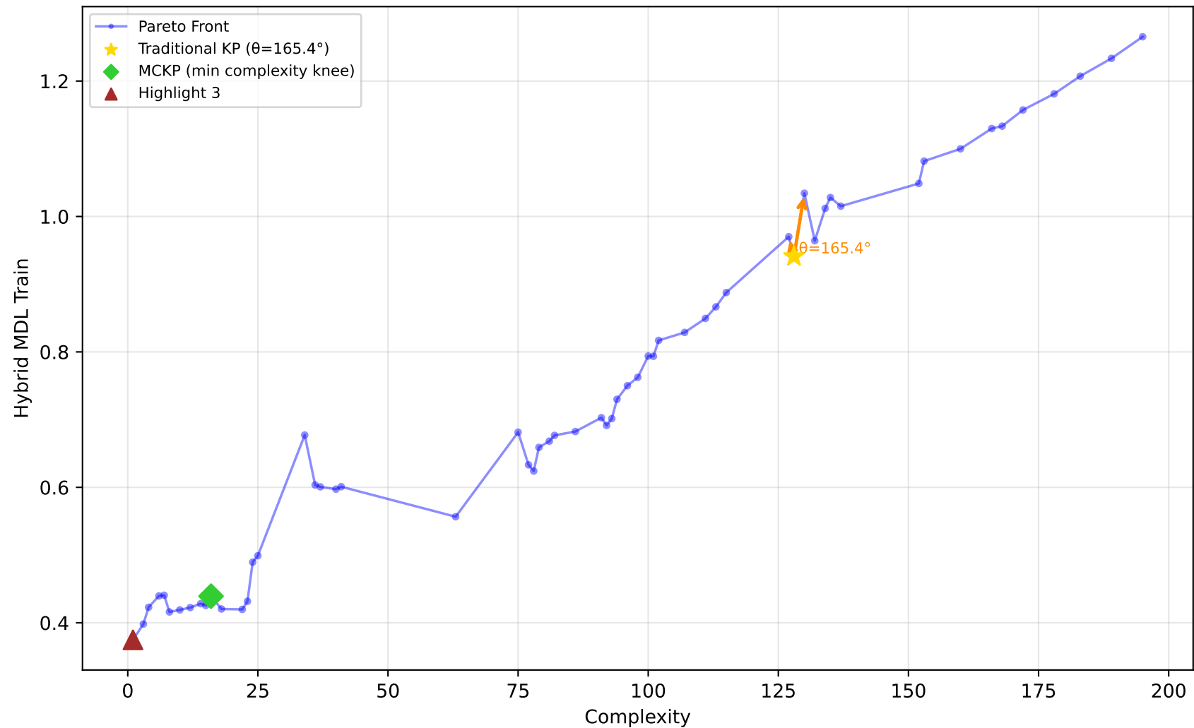
637_fri_c1_500_50 - Run 1 - MVP - Hybrid MDL Train \lambda_1=0.10, \lambda_2=0.00, \lambda_3=1.00 | Difficulty: 1.00 | Method: hmr
