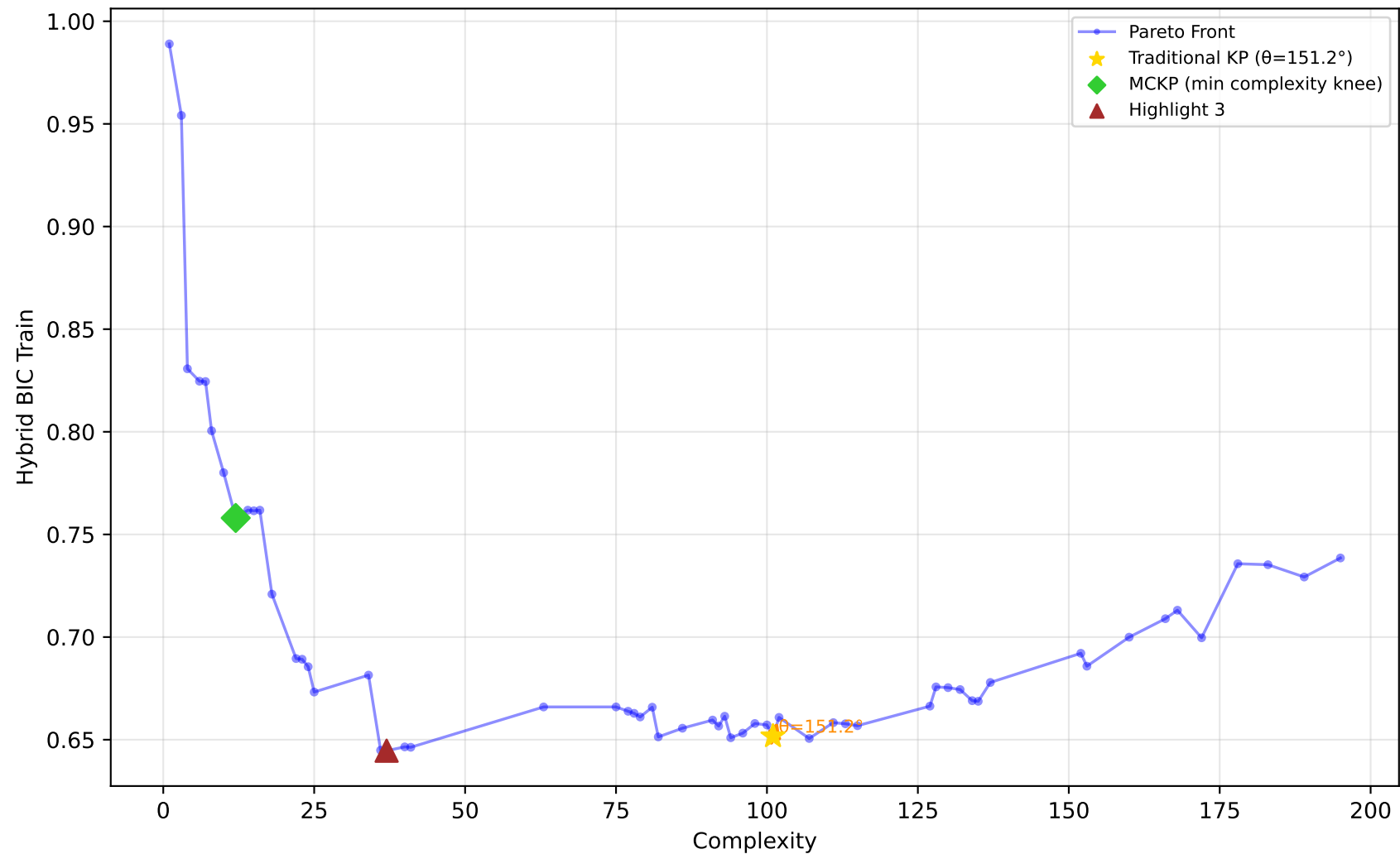
637_fri_c1_500_50 - Run 1 - SVP - Hybrid BIC Train \lambda_1=0.00, \lambda_2=0.00, \lambda_3=0.00 | Difficulty: 1.00 | Method: hmr
