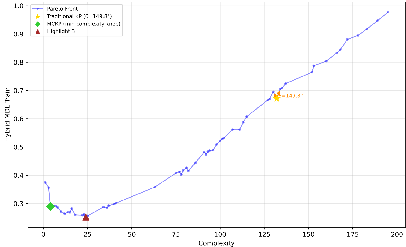
637_fri_c1_500_50 - Run 1 - SVP - Hybrid MDL Train \lambda_1=0.00, \lambda_2=0.00, \lambda_3=0.00 | Difficulty: 1.00 | Method: hmr
