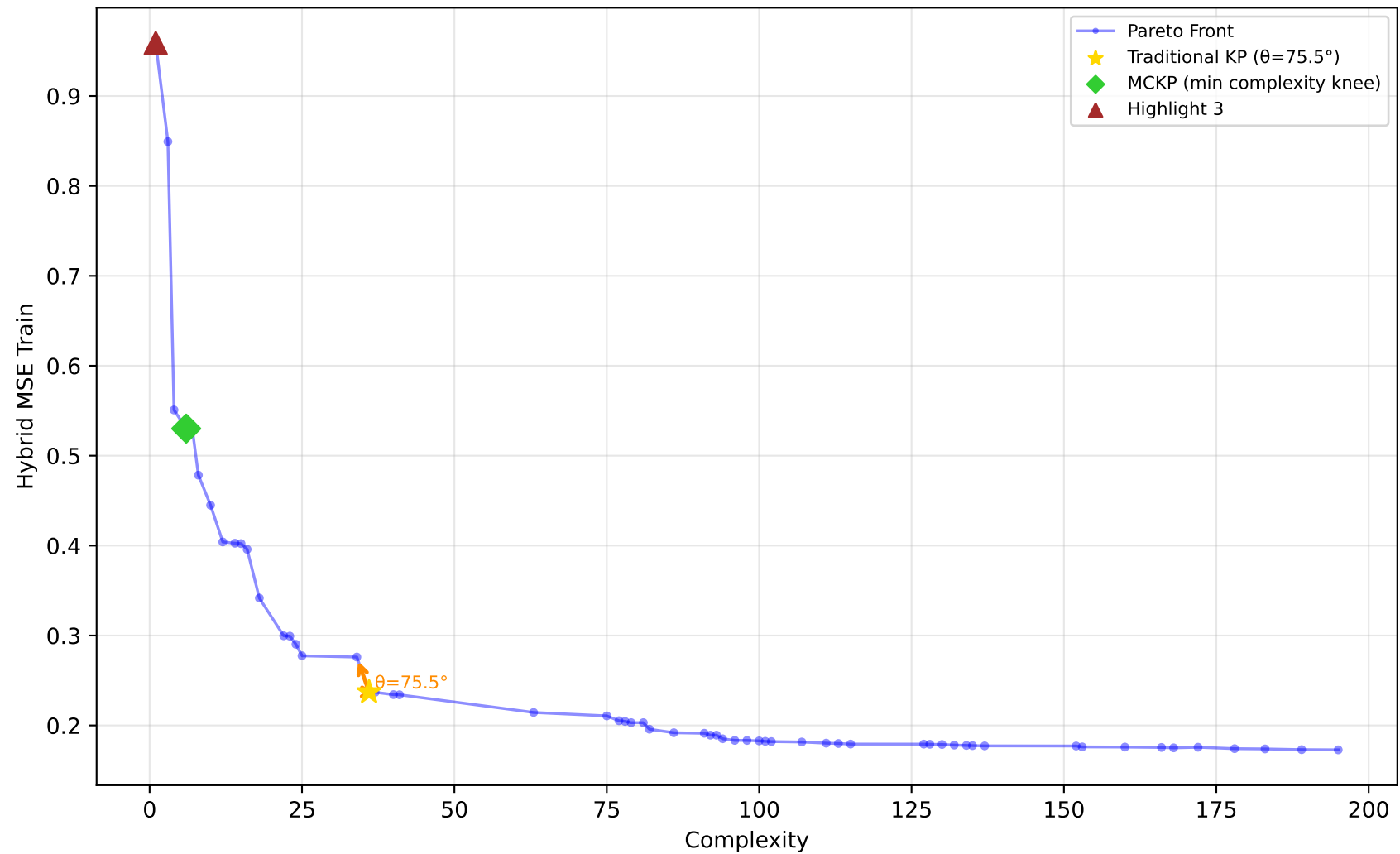
637_fri_c1_500_50 - Run 1 - SVP - Hybrid MSE Train \lambda_1=0.00, \lambda_2=0.00, \lambda_3=0.00 | Difficulty: 1.00 | Method: hmr
