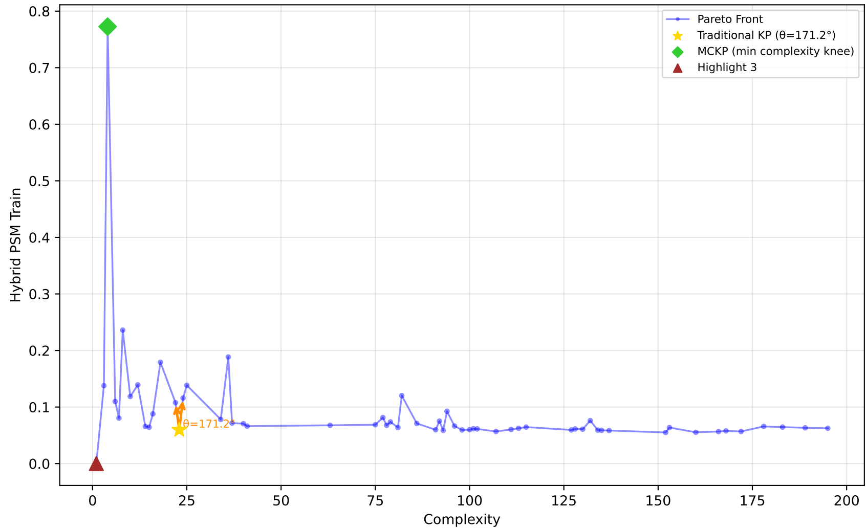
637_fri_c1_500_50 - Run 1 - SVP - Hybrid PSM Train \lambda_1=0.10, \lambda_2=0.00, \lambda_3=0.20 | Difficulty: 1.00 | Method: hmr
