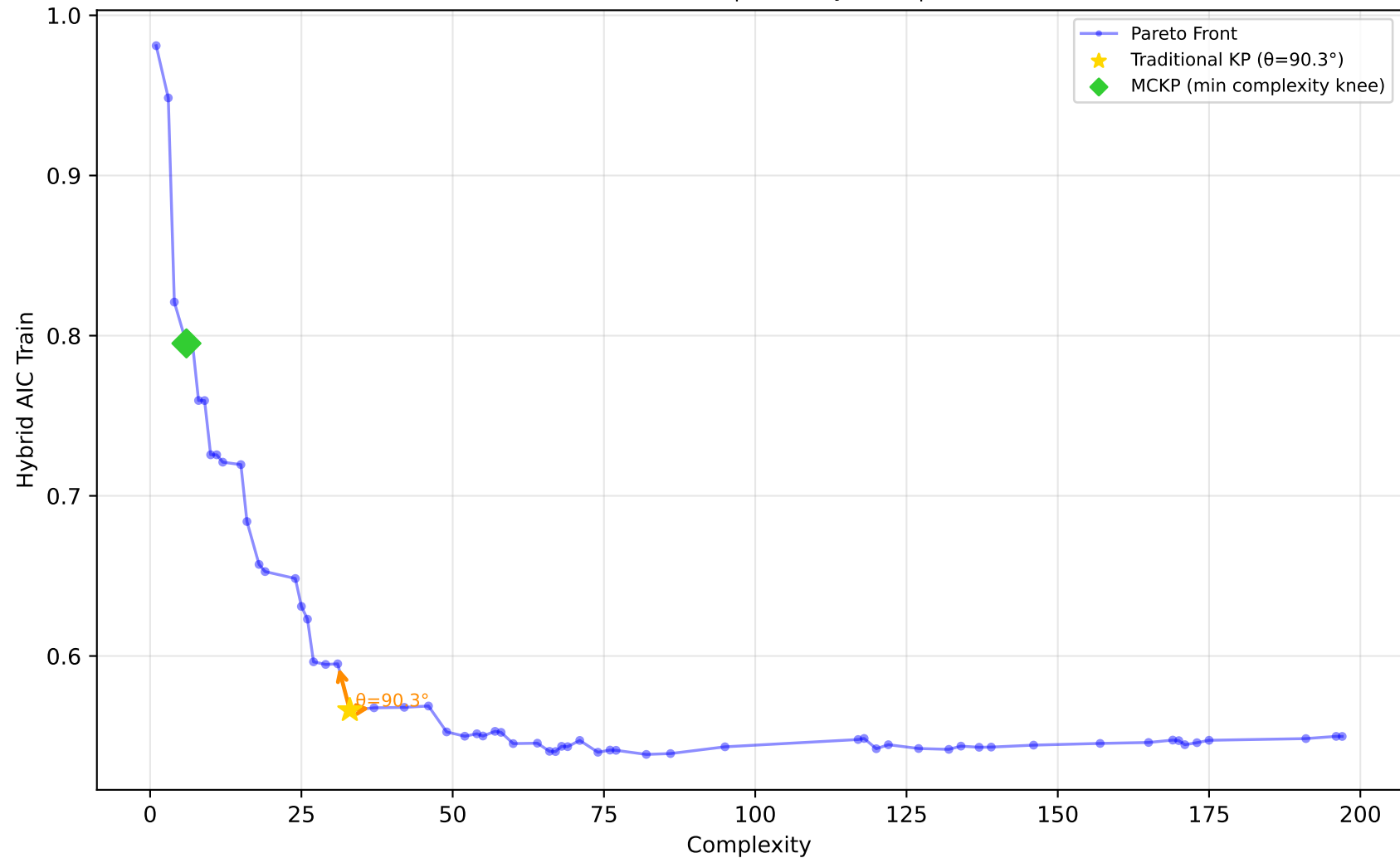
637_fri_c1_500_50 - Run 20 - MVP - Hybrid AIC Train \lambda_1=0.00, \lambda_2=0.50, \lambda_3=0.00 | Difficulty: 1.00 | Method: hmr
