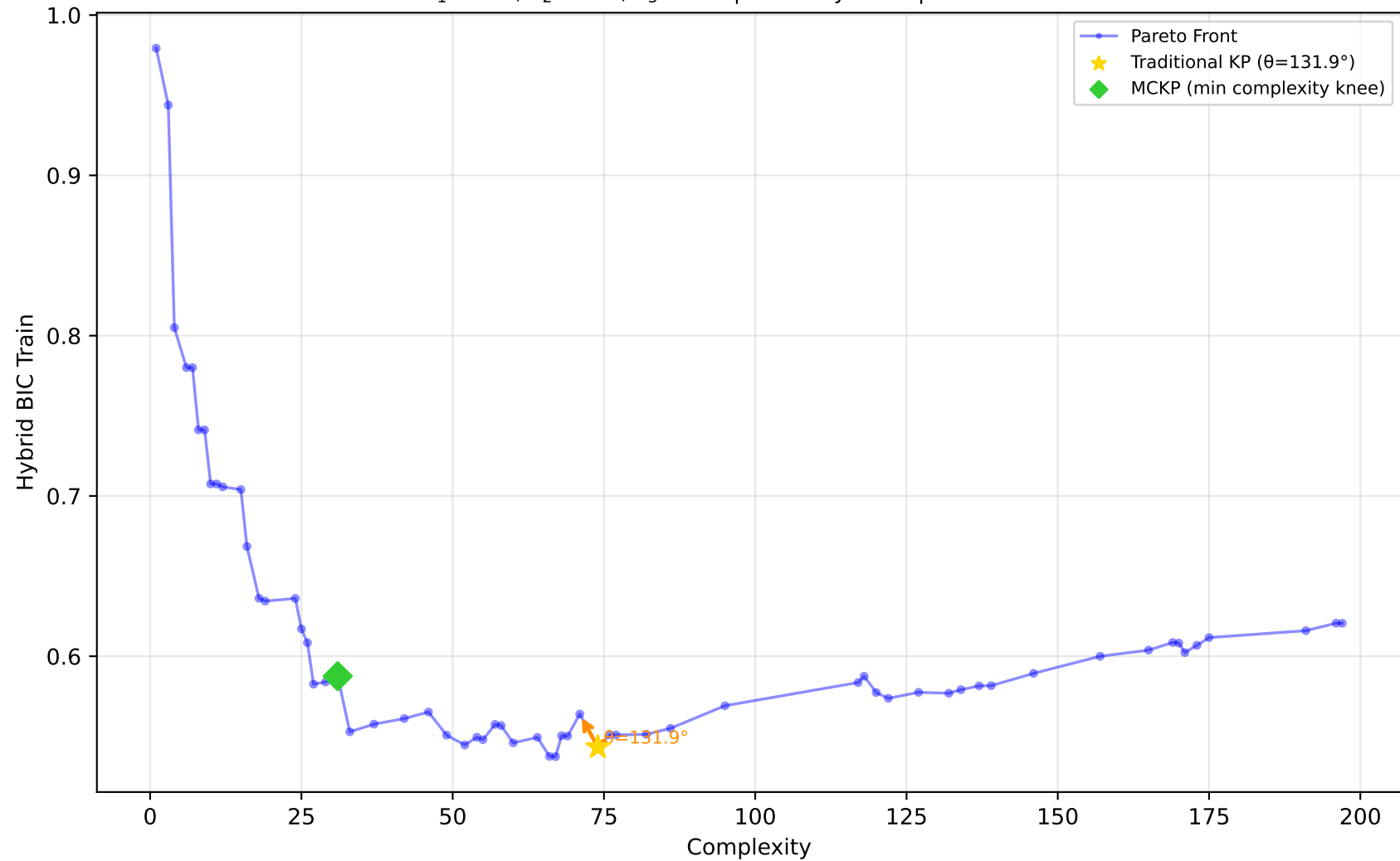
637_fri_c1_500_50 - Run 20 - MVP - Hybrid BIC Train \lambda_1=0.00, \lambda_2=0.50, \lambda_3=0.00 | Difficulty: 1.00 | Method: hmr
