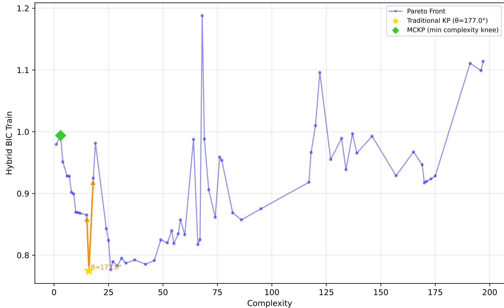
637_fri_c1_500_50 - Run 20 - MVP - Hybrid BIC Train \lambda_1=0.10, \lambda_2=0.00, \lambda_3=1.00 | Difficulty: 1.00 | Method: hmr
