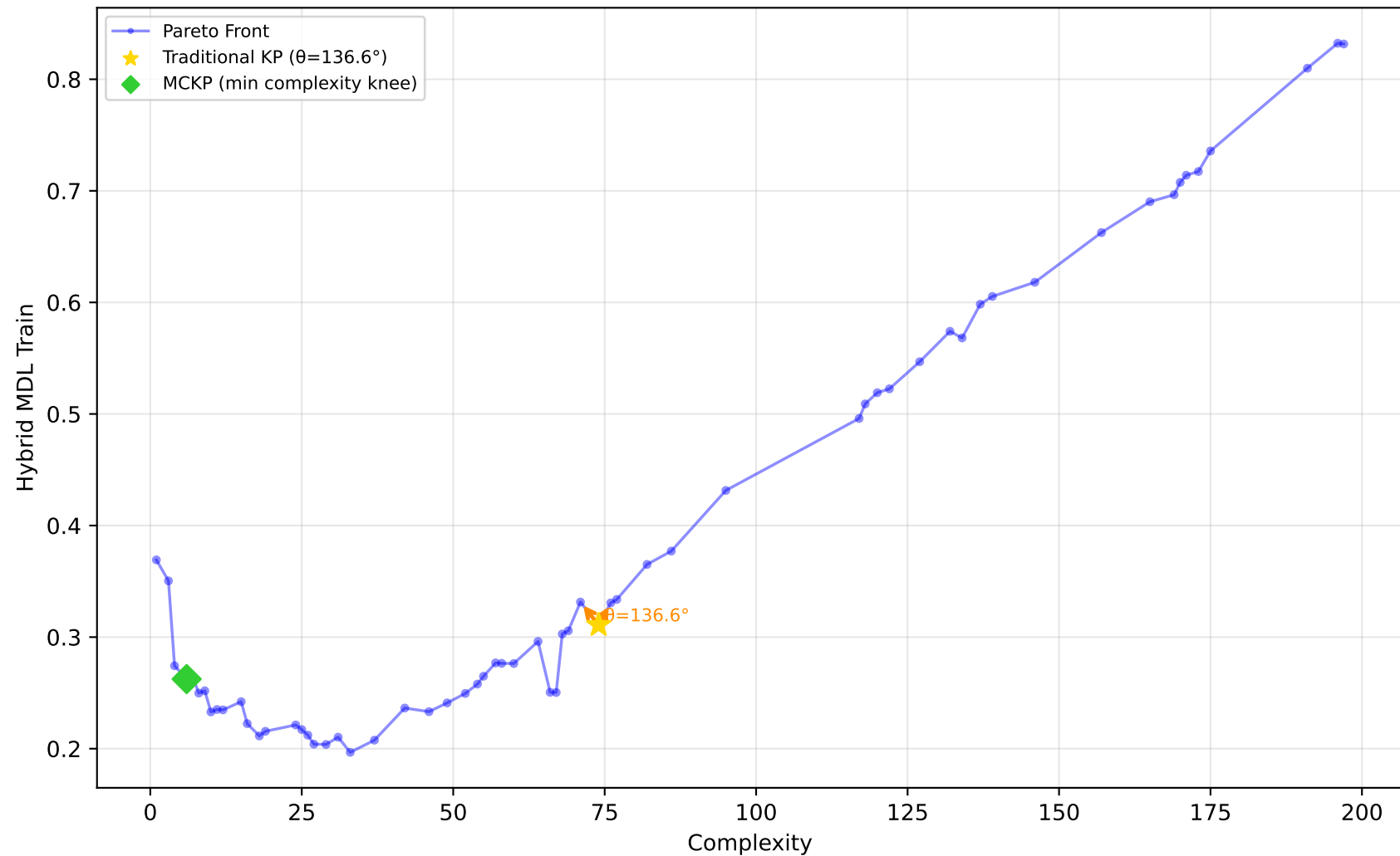
637_fri_c1_500_50 - Run 20 - MVP - Hybrid MDL Train \lambda_1=0.00, \bar{\lambda}_2=0.50, \bar{\lambda}_3=0.00 | Difficulty: 1.00 | Method: hmr
