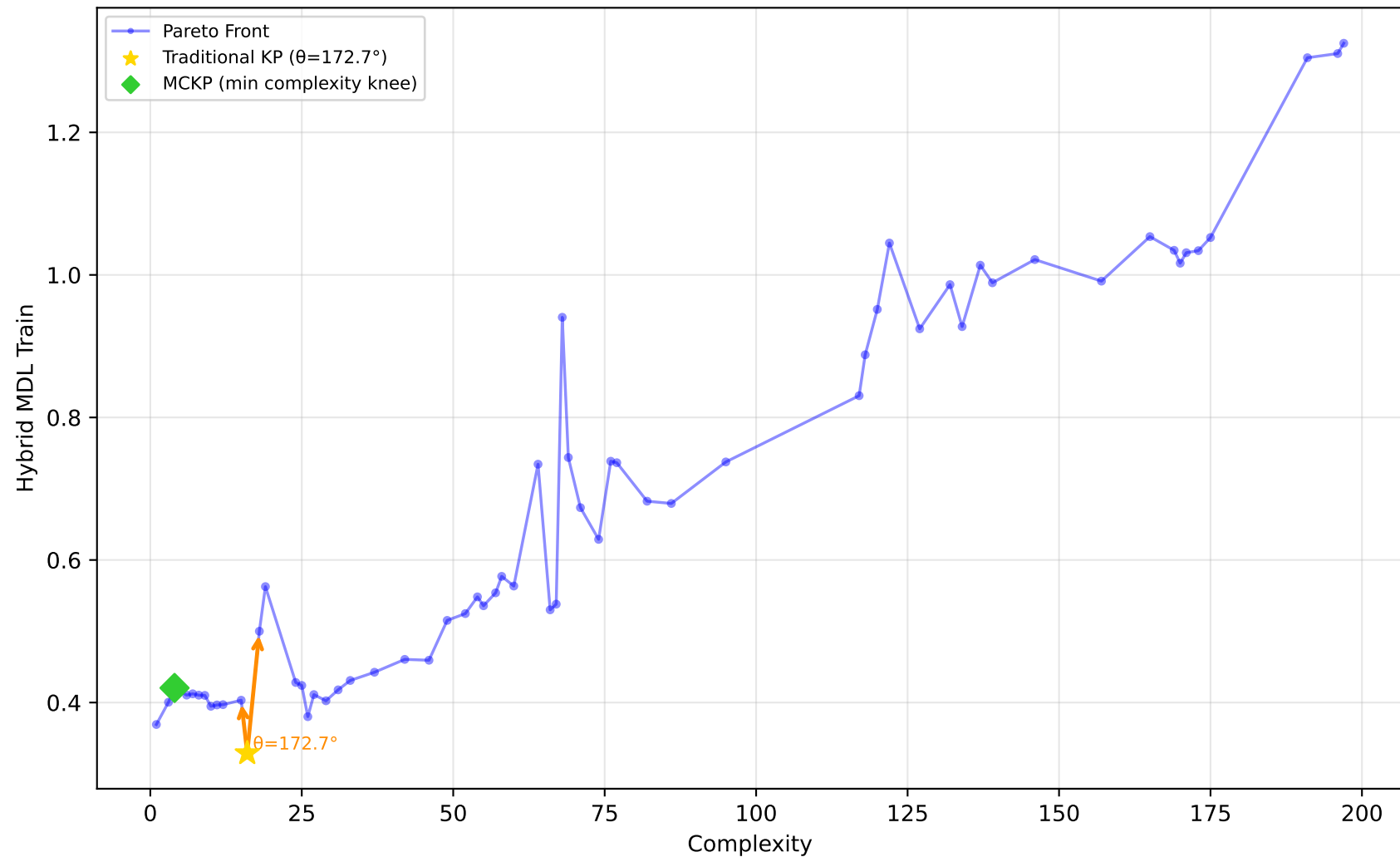
637_fri_c1_500_50 - Run 20 - MVP - Hybrid MDL Train \lambda_1=0.10, \bar{\lambda}_2=0.00, \bar{\lambda}_3=1.00 | Difficulty: 1.00 | Method: hmr
