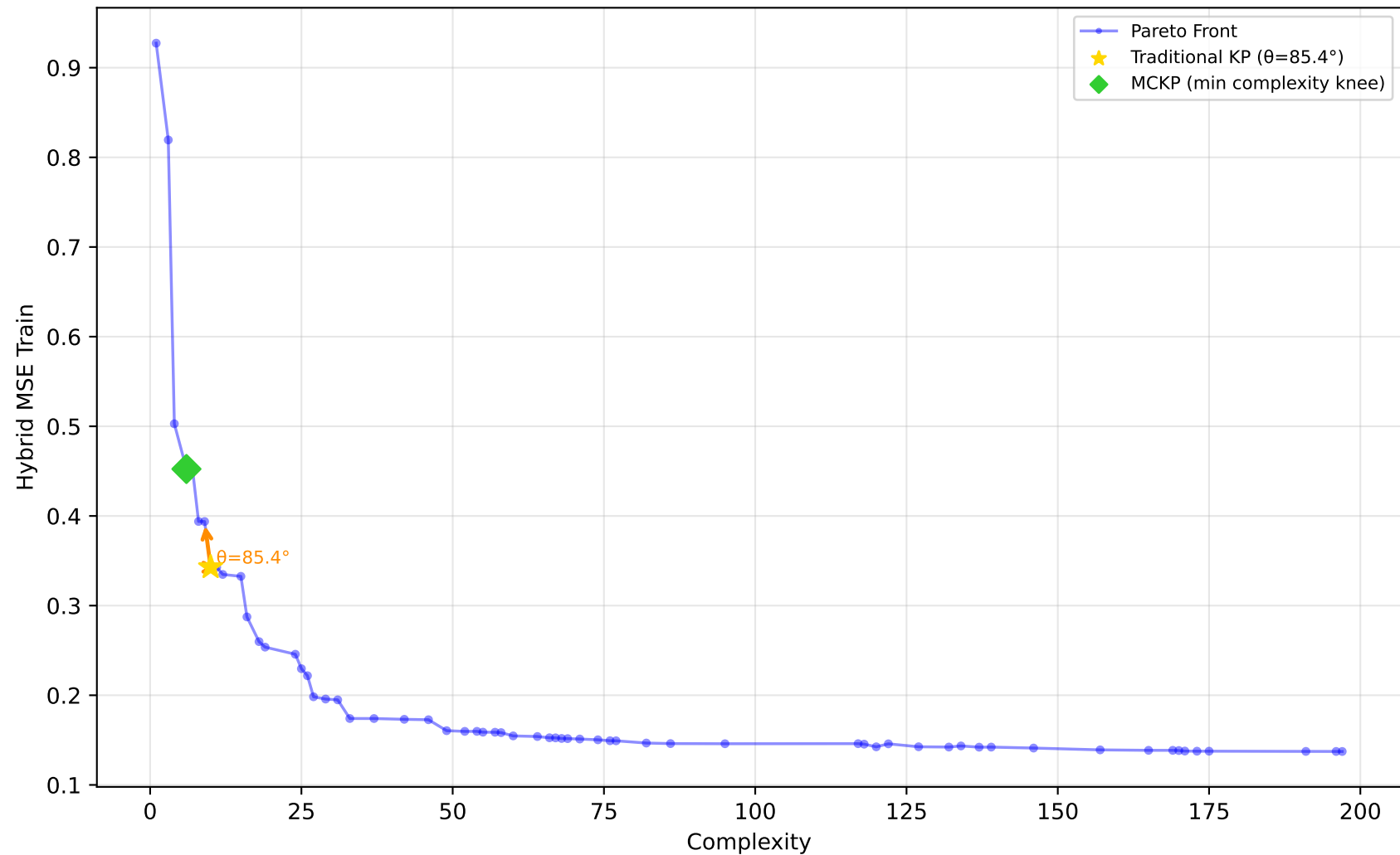
637_fri_c1_500_50 - Run 20 - MVP - Hybrid MSE Train \lambda_1=0.00, \lambda_2=0.50, \lambda_3=0.00 | Difficulty: 1.00 | Method: hmr
