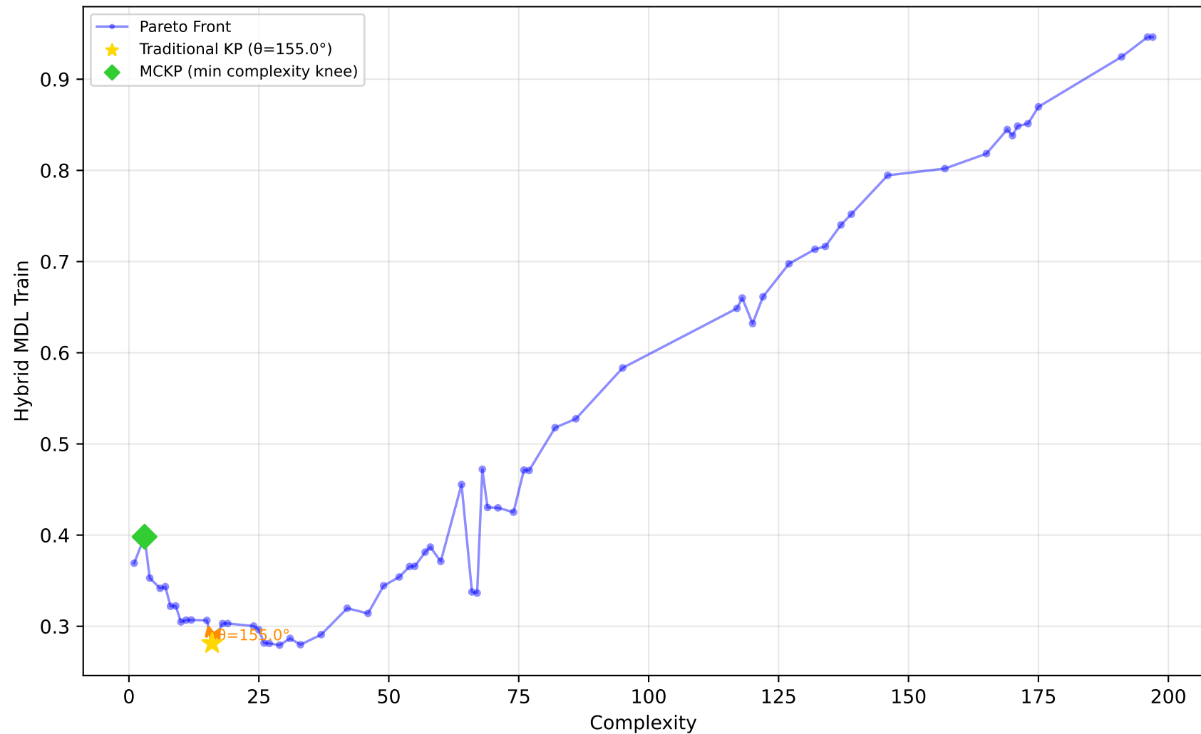
637_fri_c1_500_50 - Run 20 - SVP - Hybrid MDL Train \lambda_1=0.10, \lambda_2=0.00, \lambda_3=0.20 | Difficulty: 1.00 | Method: hmr
