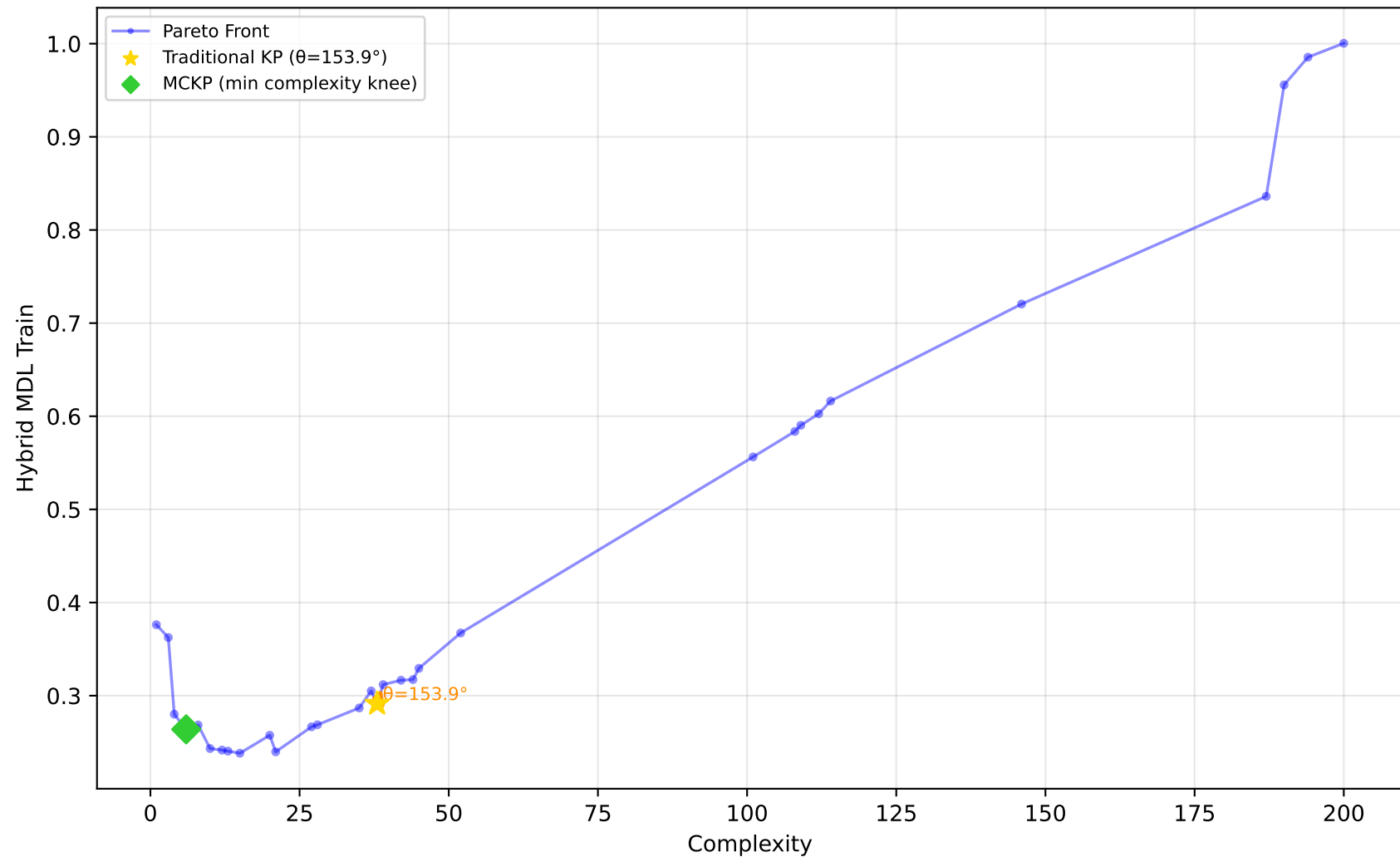
637_fri_c1_500_50 - Run 21 - MVP - Hybrid MDL Train \lambda_1=0.00, \bar{\lambda}_2=0.50, \bar{\lambda}_3=0.00 | Difficulty: 1.00 | Method: hmr
