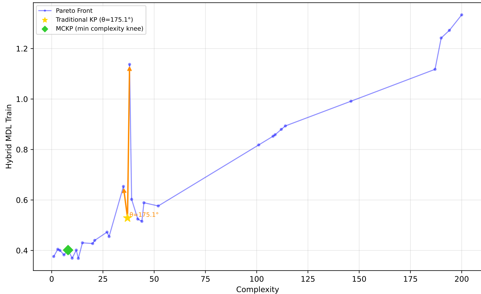
637_fri_c1_500_50 - Run 21 - MVP - Hybrid MDL Train \lambda_1=0.10, \bar{\lambda}_2=0.00, \bar{\lambda}_3=1.00 | Difficulty: 1.00 | Method: hmr
