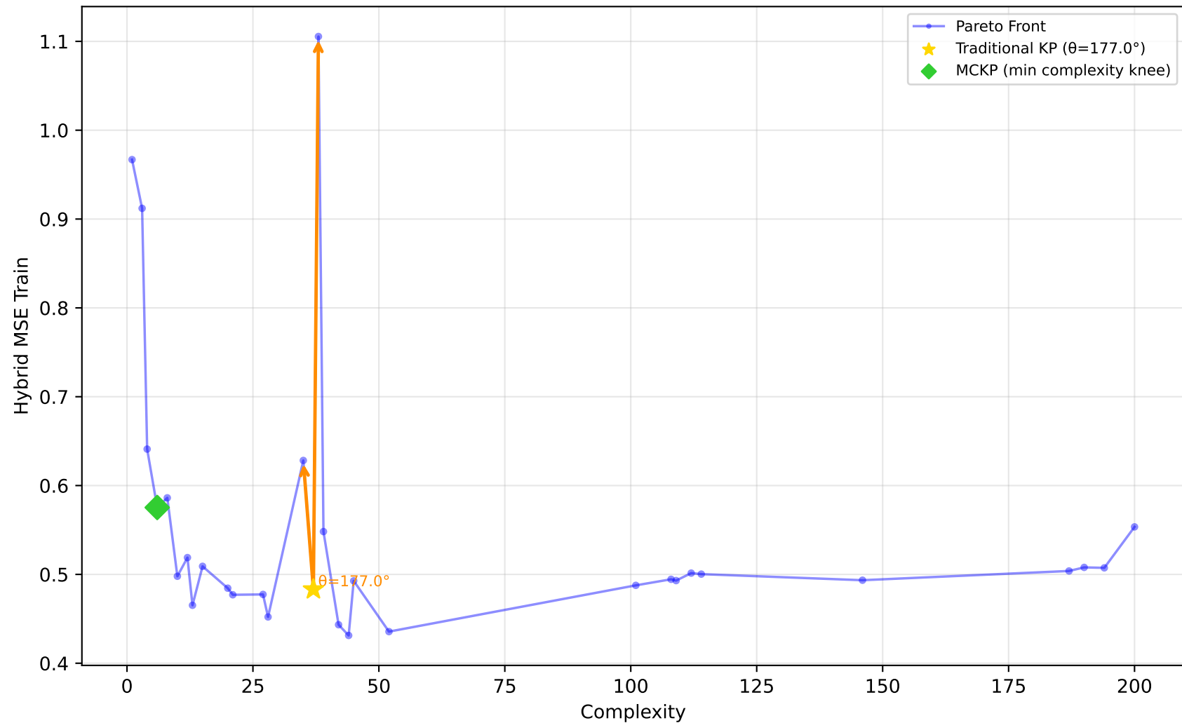
637_fri_c1_500_50 - Run 21 - MVP - Hybrid MSE Train \lambda_1=0.10, \bar{\lambda}_2=0.00, \bar{\lambda}_3=1.00 | Difficulty: 1.00 | Method: hmr
