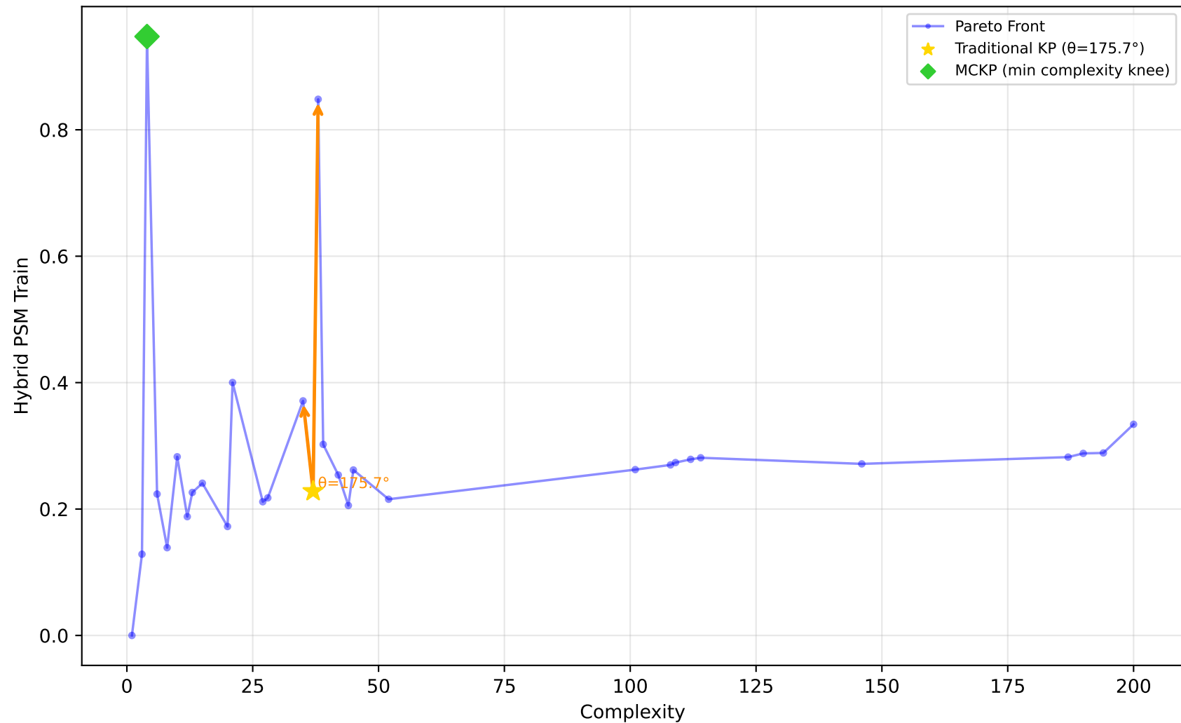
637_fri_c1_500_50 - Run 21 - MVP - Hybrid PSM Train \lambda_1=0.10, \lambda_2=0.00, \lambda_3=1.00 | Difficulty: 1.00 | Method: hmr
