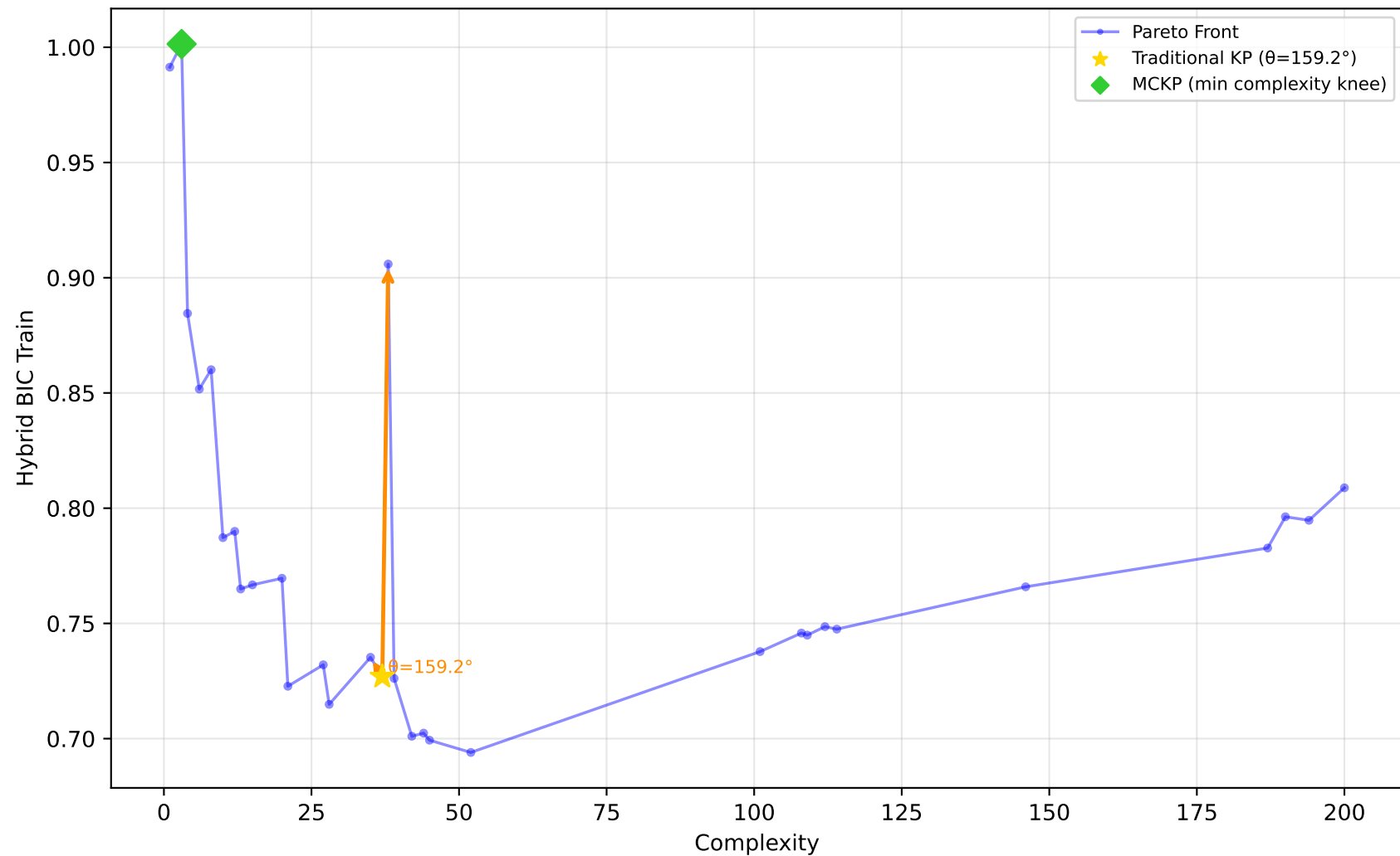
637_fri_c1_500_50 - Run 21 - SVP - Hybrid BIC Train \lambda_1=0.10, \lambda_2=0.00, \lambda_3=0.20 | Difficulty: 1.00 | Method: hmr
