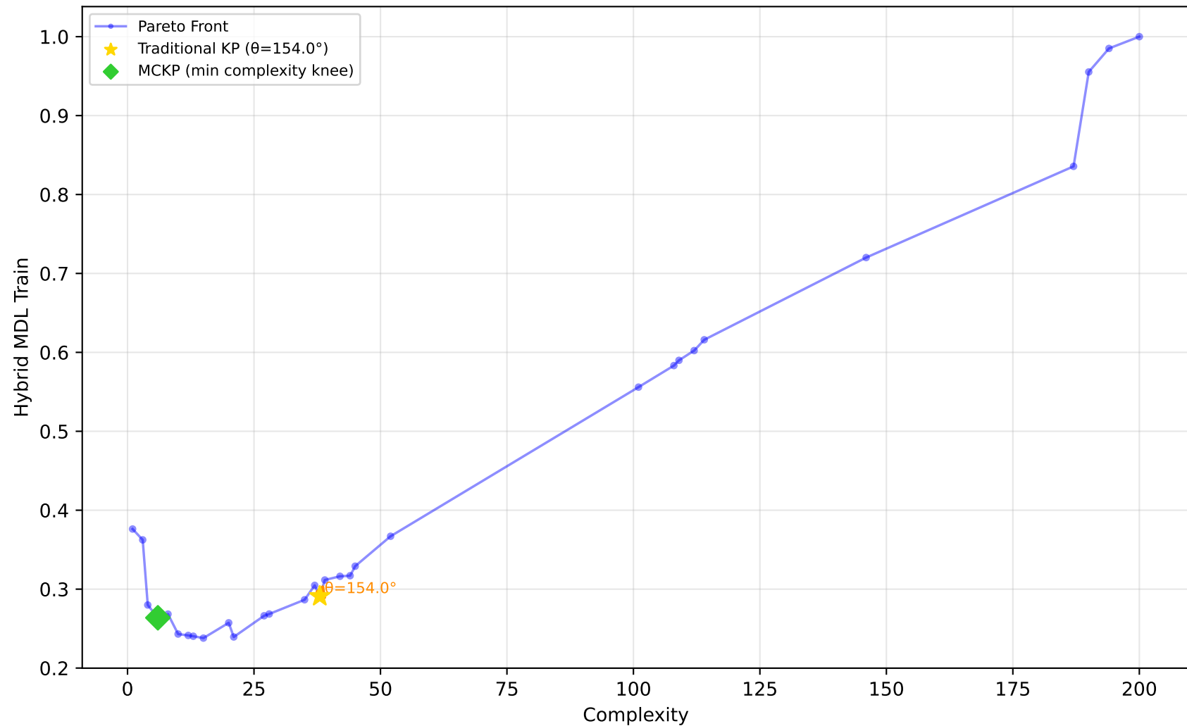
637_fri_c1_500_50 - Run 21 - SVP - Hybrid MDL Train \lambda_1=0.00, \lambda_2=0.00, \lambda_3=0.00 | Difficulty: 1.00 | Method: hmr
