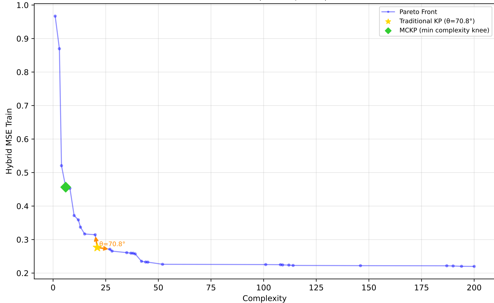
637_fri_c1_500_50 - Run 21 - SVP - Hybrid MSE Train \lambda_1=0.00, \lambda_2=0.00, \lambda_3=0.00 | Difficulty: 1.00 | Method: hmr
