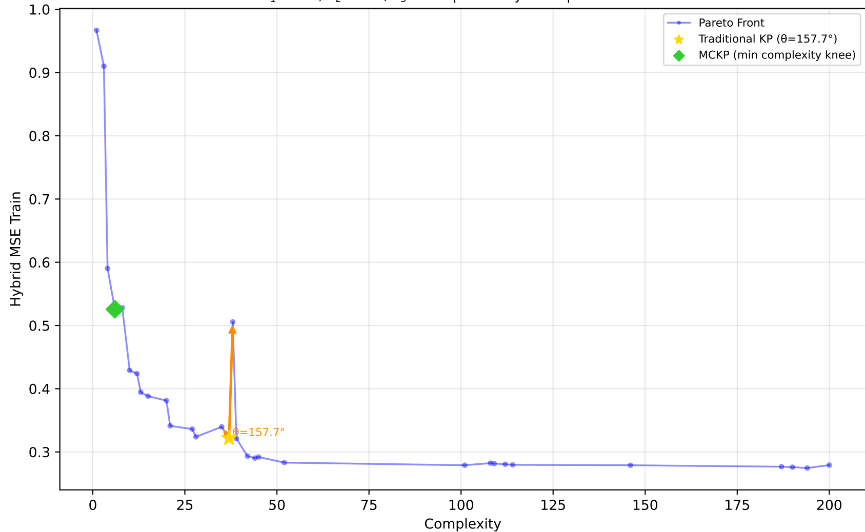
637_fri_c1_500_50 - Run 21 - SVP - Hybrid MSE Train \lambda_1=0.10, \lambda_2=0.00, \lambda_3=0.20 | Difficulty: 1.00 | Method: hmr
