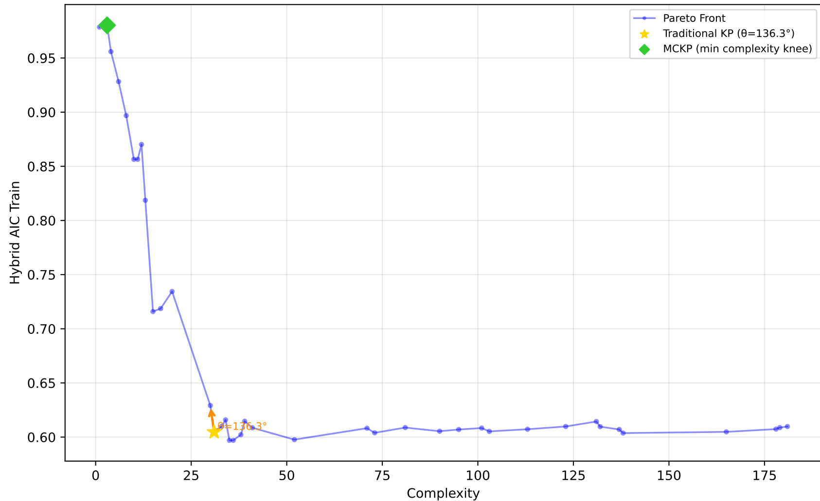
637_fri_c1_500_50 - Run 22 - MVP - Hybrid AIC Train \lambda_1=0.10, \lambda_2=0.00, \lambda_3=1.00 | Difficulty: 1.00 | Method: hmr
