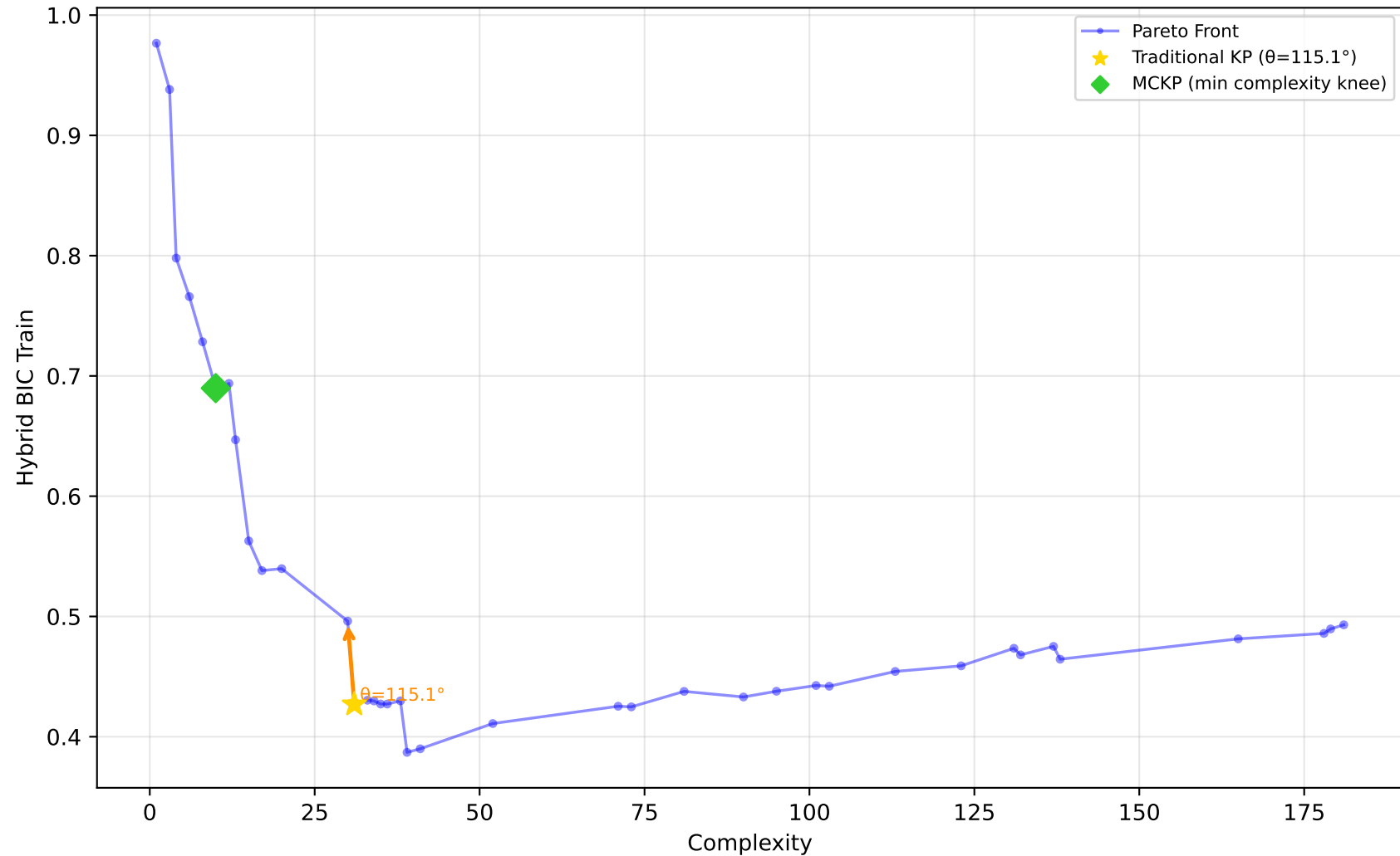
637_fri_c1_500_50 - Run 22 - MVP - Hybrid BIC Train \lambda_1=0.00, \lambda_2=0.50, \lambda_3=0.00 | Difficulty: 1.00 | Method: hmr
