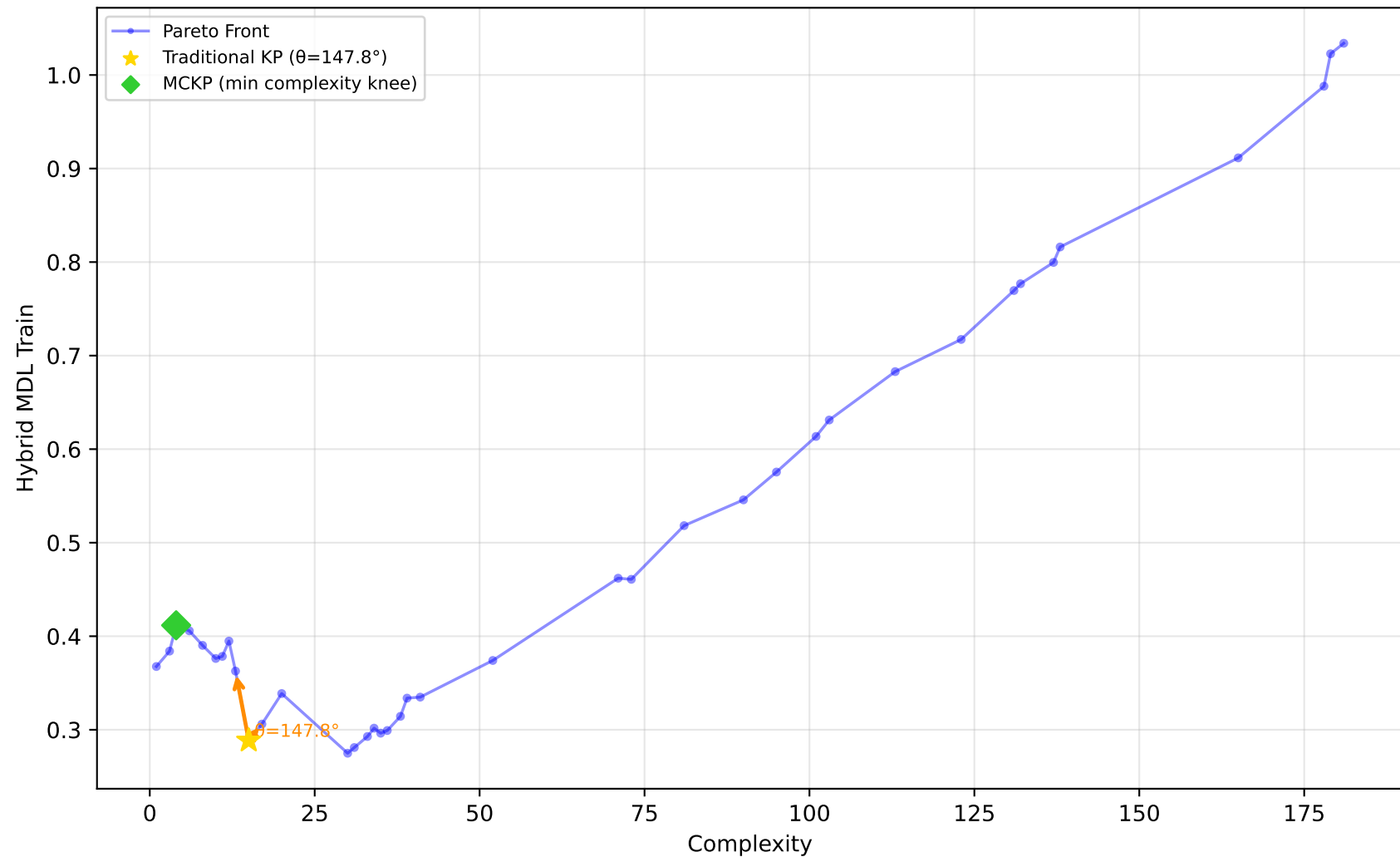
637_fri_c1_500_50 - Run 22 - MVP - Hybrid MDL Train \lambda_1=0.10, \bar{\lambda}_2=0.00, \bar{\lambda}_3=1.00 | Difficulty: 1.00 | Method: hmr
