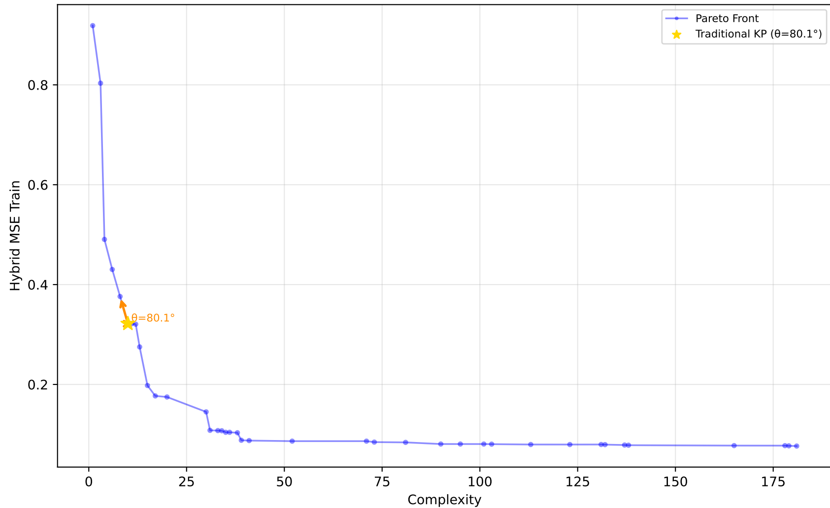
637_fri_c1_500_50 - Run 22 - MVP - Hybrid MSE Train \lambda_1=0.00, \bar{\lambda}_2=0.50, \lambda_3=0.00 | Difficulty: 1.00 | Method: hmr
