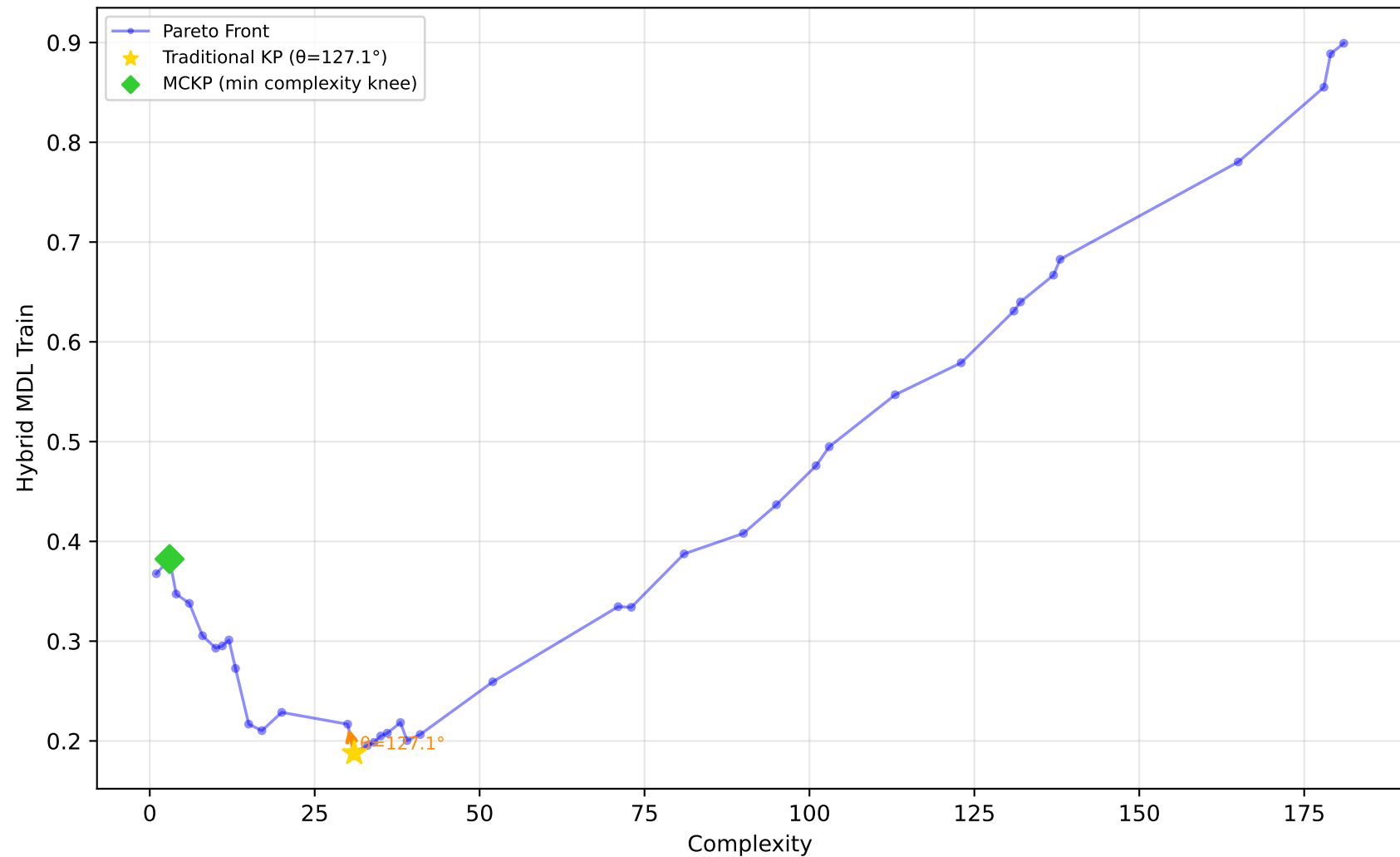
637_fri_c1_500_50 - Run 22 - SVP - Hybrid MDL Train \lambda_1=0.10, \lambda_2=0.00, \lambda_3=0.20 | Difficulty: 1.00 | Method: hmr
