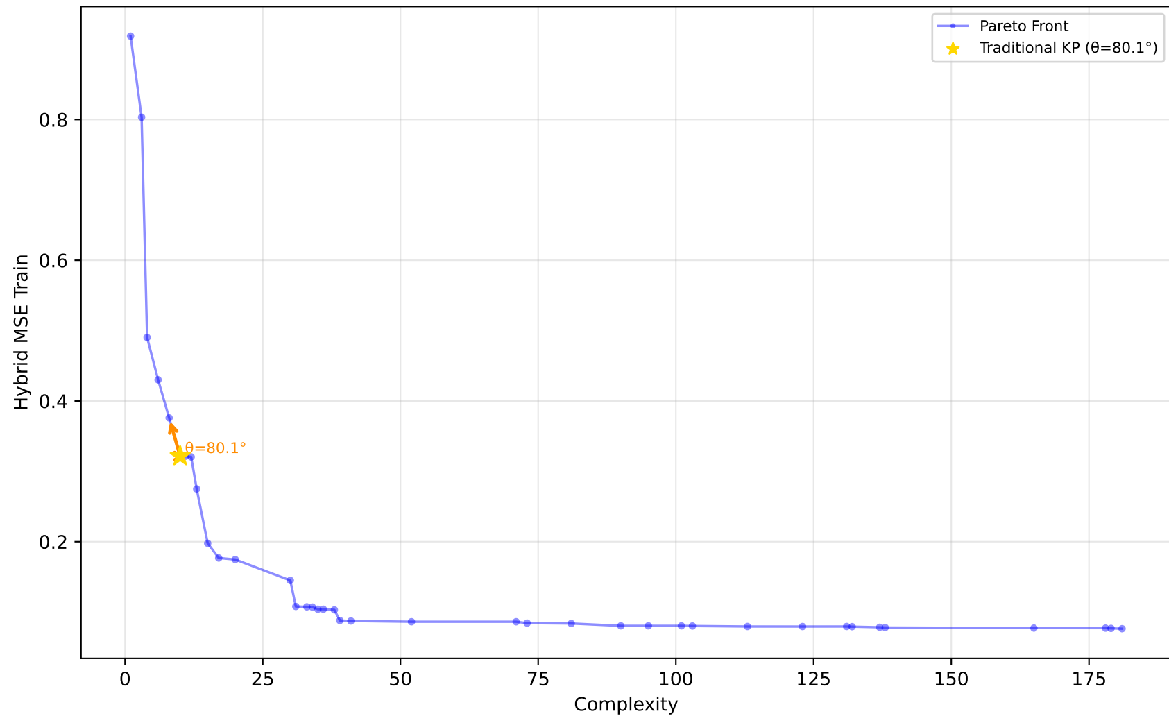
637_fri_c1_500_50 - Run 22 - SVP - Hybrid MSE Train \lambda_1=0.00, \lambda_2=0.00, \lambda_3=0.00 | Difficulty: 1.00 | Method: hmr
