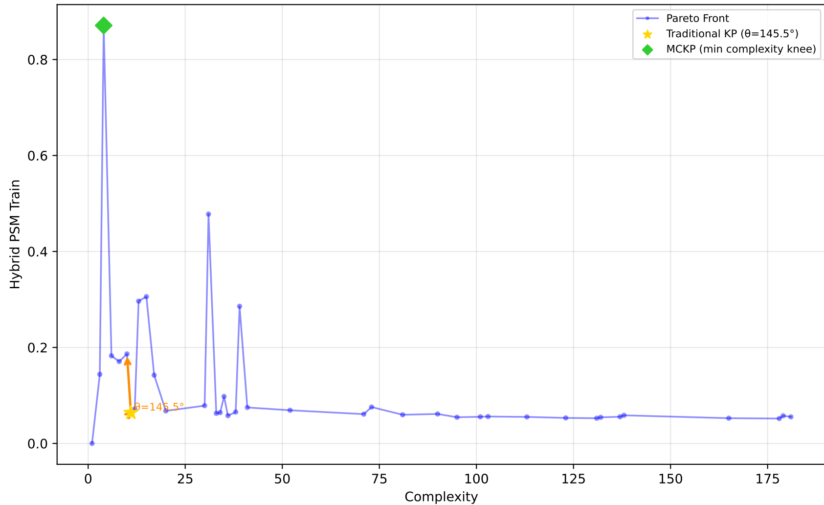
637_fri_c1_500_50 - Run 22 - SVP - Hybrid PSM Train \lambda_1=0.10, \lambda_2=0.00, \lambda_3=0.20 | Difficulty: 1.00 | Method: hmr
