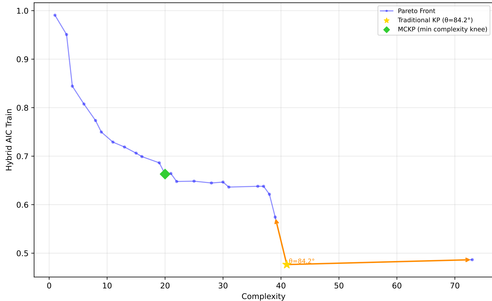
637_fri_c1_500_50 - Run 23 - MVP - Hybrid AIC Train \lambda_1=0.00 , \lambda_2=0.50 , \lambda_3=0.00 | Difficulty: 1.00 | Method: hmr
