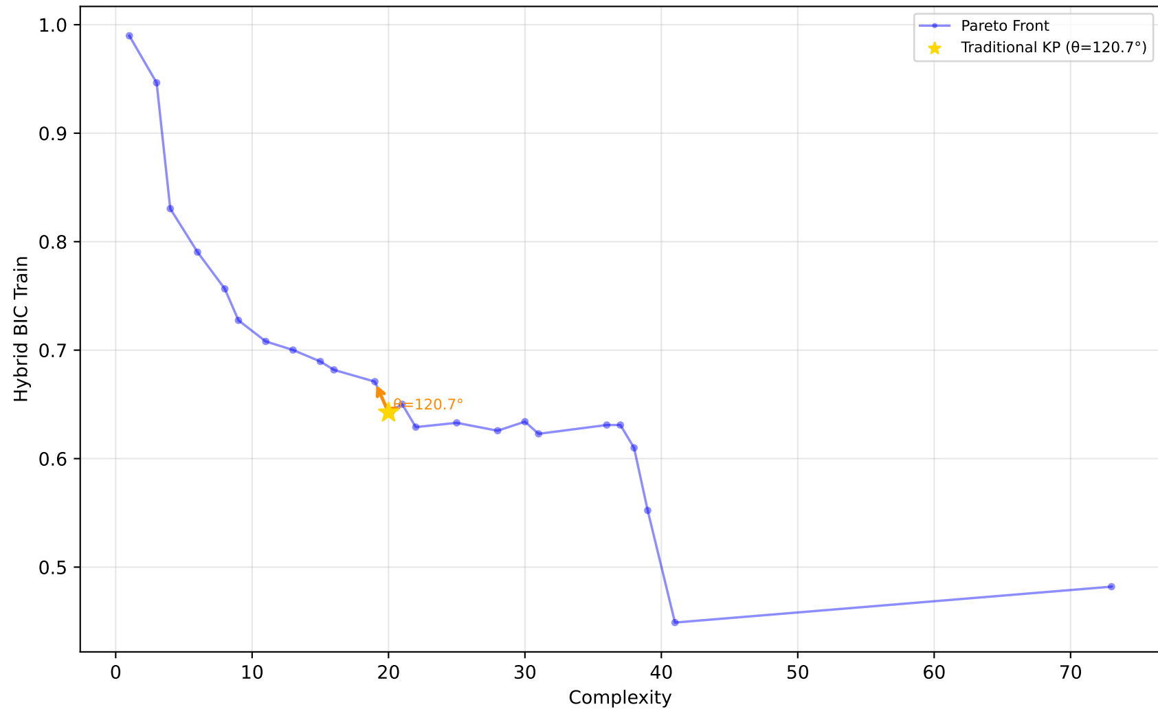
637_fri_c1_500_50 - Run 23 - MVP - Hybrid BIC Train \lambda_1=0.00, \lambda_2=0.50, \lambda_3=0.00 | Difficulty: 1.00 | Method: hmr
