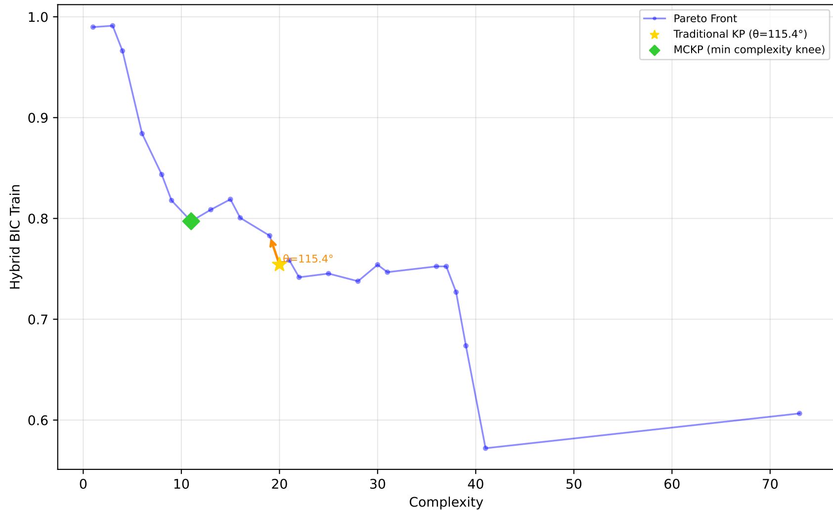
637_fri_c1_500_50 - Run 23 - MVP - Hybrid BIC Train \lambda_1=0.10, \lambda_2=0.00, \lambda_3=1.00 | Difficulty: 1.00 | Method: hmr
