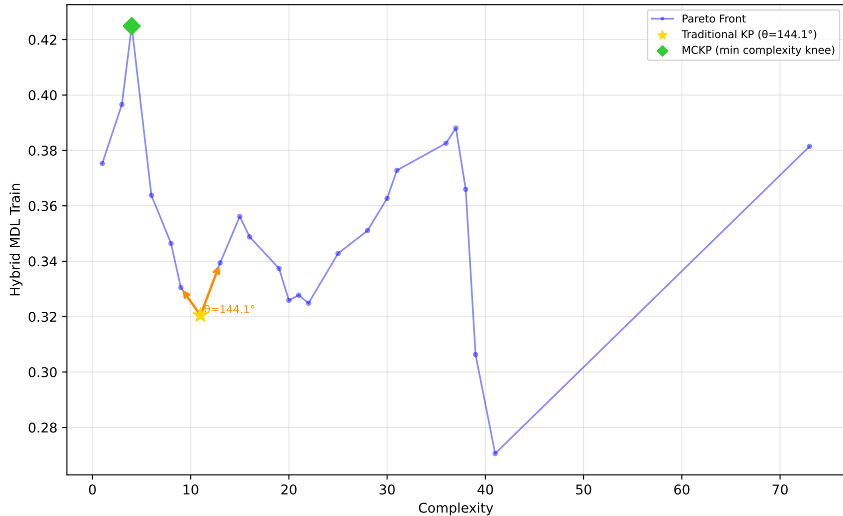
637_fri_c1_500_50 - Run 23 - MVP - Hybrid MDL Train \lambda_1=0.10, \lambda_2=0.00, \lambda_3=1.00 | Difficulty: 1.00 | Method: hmr
