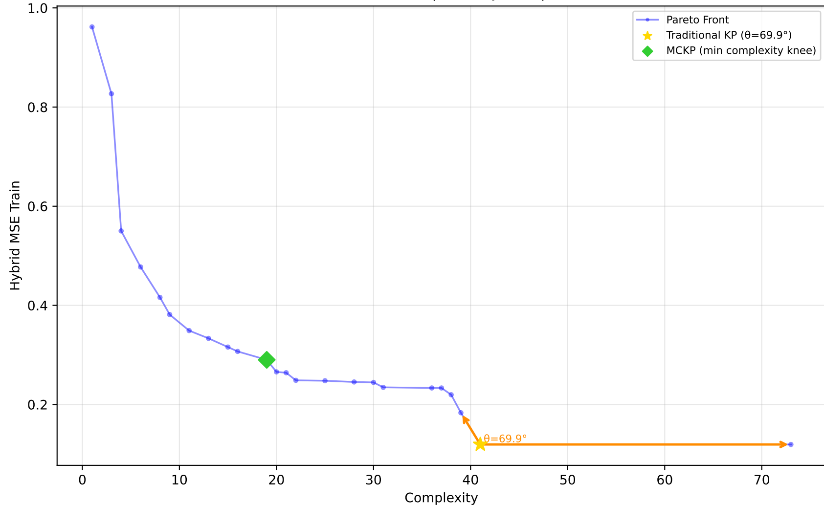
637_fri_c1_500_50 - Run 23 - MVP - Hybrid MSE Train \lambda_1=0.00, \bar{\lambda}_2=0.50, \lambda_3=0.00 | Difficulty: 1.00 | Method: hmr
