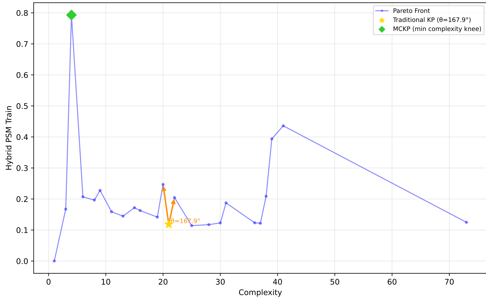
637_fri_c1_500_50 - Run 23 - MVP - Hybrid PSM Train \lambda_1=0.10, \bar{\lambda}_2=0.00, \lambda_3=1.00 | Difficulty: 1.00 | Method: hmr
