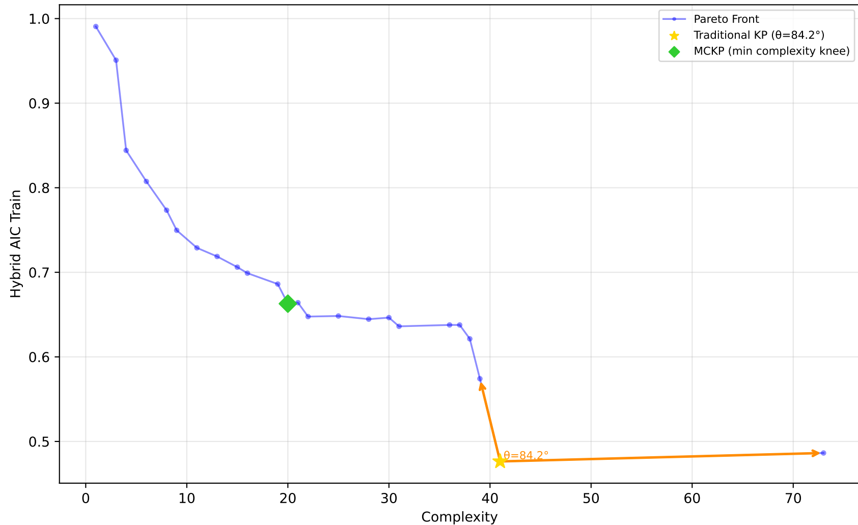
637_fri_c1_500_50 - Run 23 - SVP - Hybrid AIC Train \lambda_1=0.00, \lambda_2=0.00, \lambda_3=0.00 | Difficulty: 1.00 | Method: hmr
