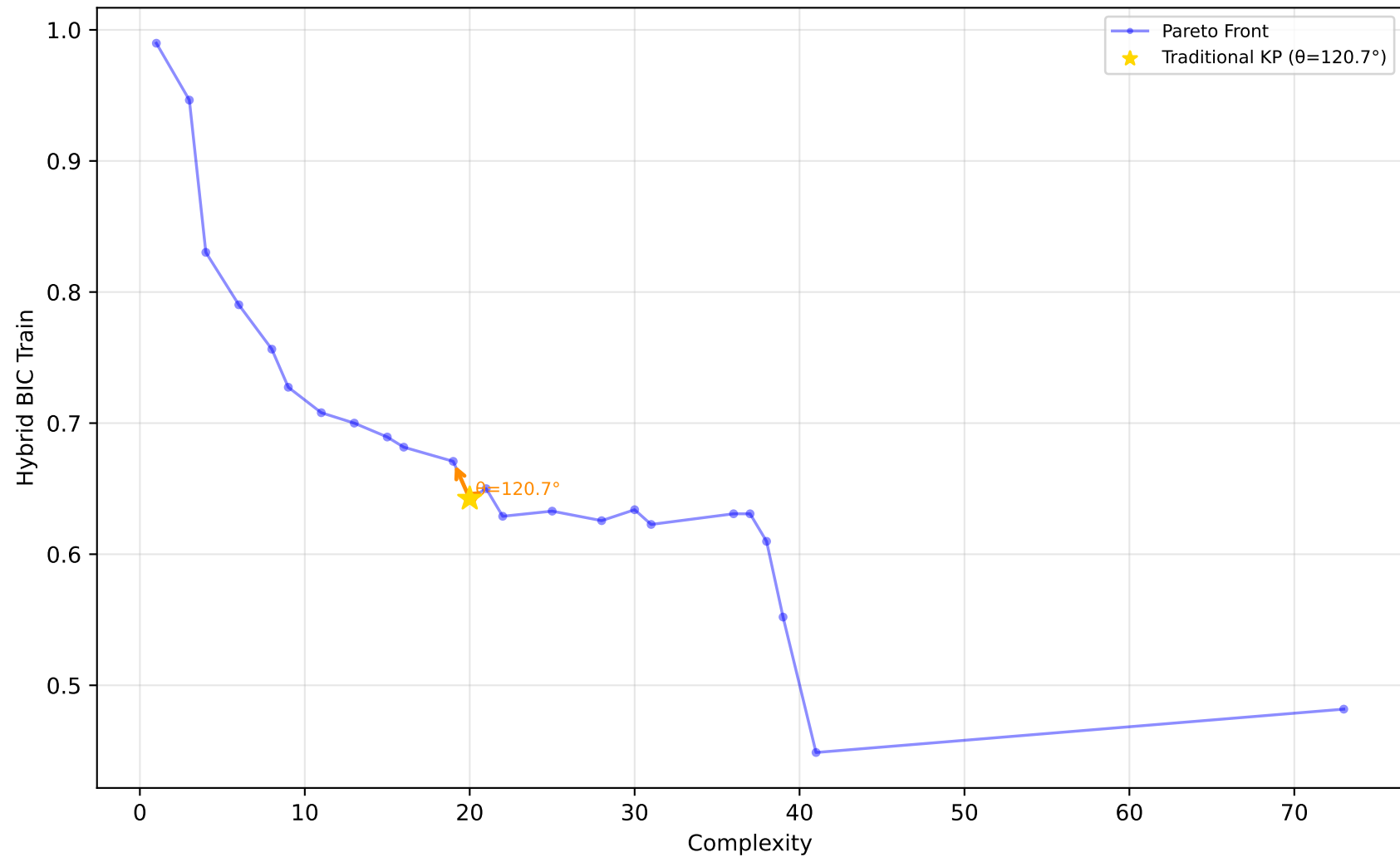
637_fri_c1_500_50 - Run 23 - SVP - Hybrid BIC Train \lambda_1=0.00, \lambda_2=0.00, \lambda_3=0.00 | Difficulty: 1.00 | Method: hmr
