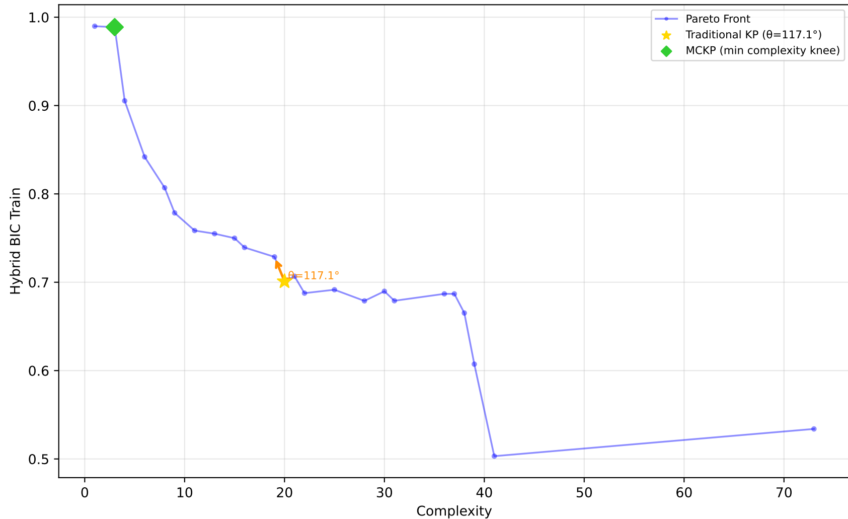
637_fri_c1_500_50 - Run 23 - SVP - Hybrid BIC Train \lambda_1=0.10, \lambda_2=0.00, \lambda_3=0.20 | Difficulty: 1.00 | Method: hmr
