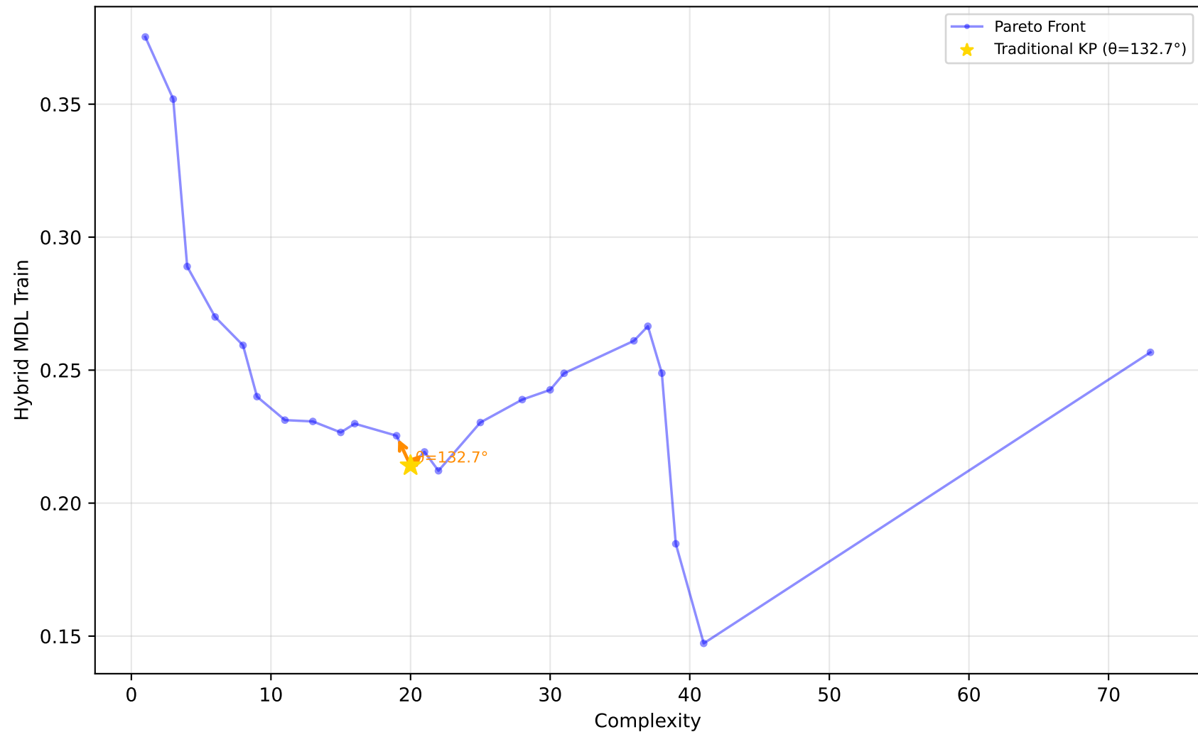
637_fri_c1_500_50 - Run 23 - SVP - Hybrid MDL Train \lambda_1=0.00, \lambda_2=0.00, \lambda_3=0.00 | Difficulty: 1.00 | Method: hmr
